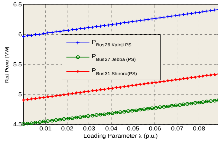
Figure 6. Increase in real power Supply at the PV buses for Area 1 to Area 2 Transfer.
