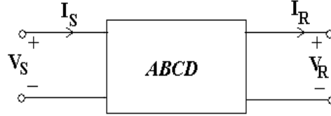
Figure 3. Two port representation of a Transmission line.
