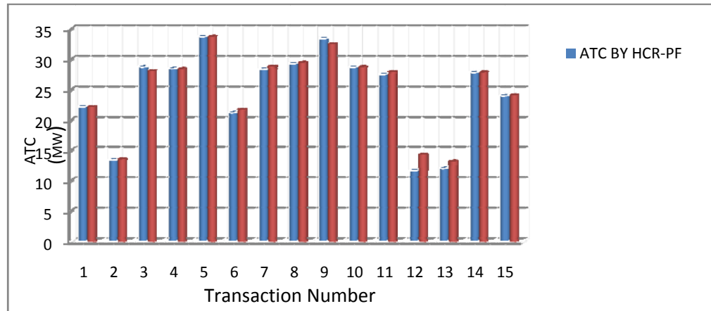
Figure 4. Comparison between HCR-PF and Wu's Method in IEEE 30 bus network for Bus 14 to bus 21 transaction.
