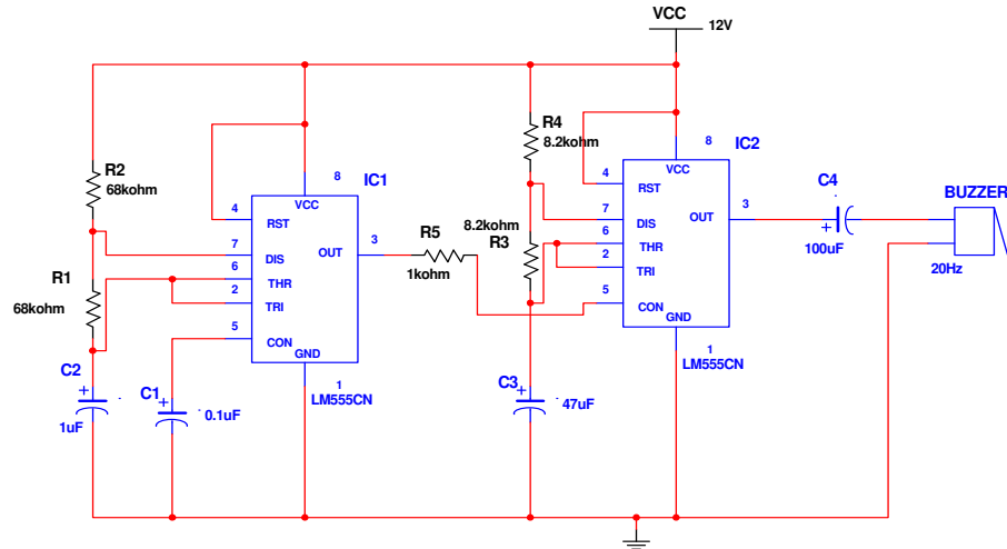
Fig. 5: circuit diagram of the tone generation unit
