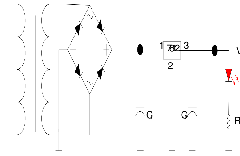
Fig. 2: The power supply unit
