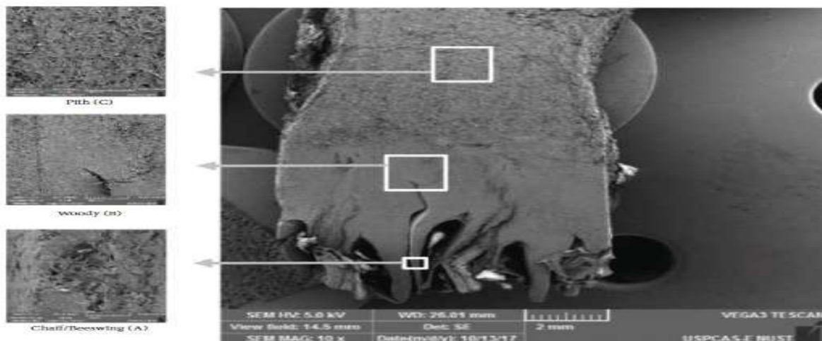
Figure 1: Scanning Electron Microscopy analysis of Corn Cob Ash (CCA)
