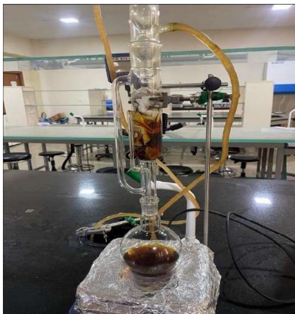
Figure 2: Extraction of crude oil from SACHPC Filter
