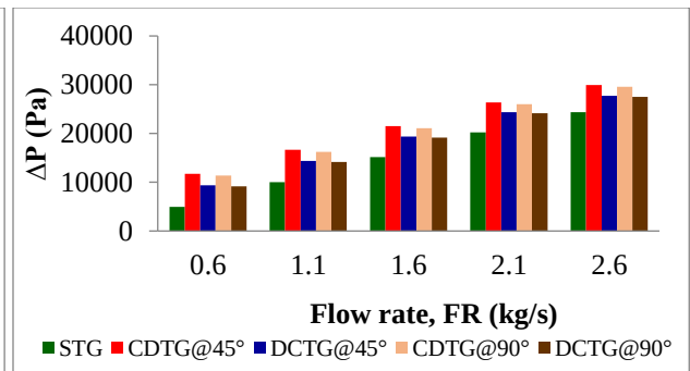
Fig. 5: Shell-side pressure drop in the selected STHEs
