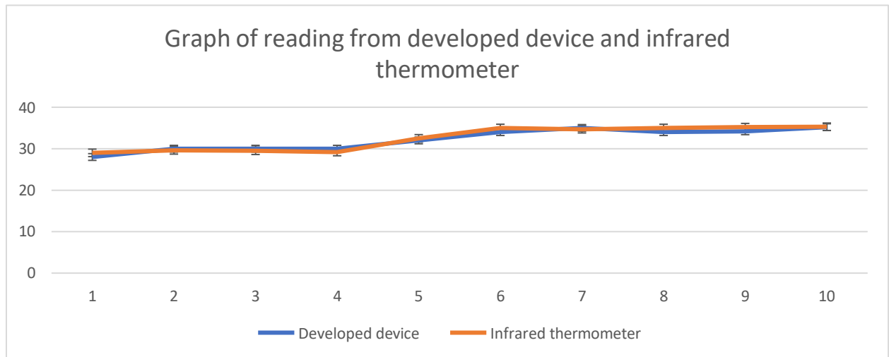
Fig 13 Temperature reading against developed and infrared thermometer
