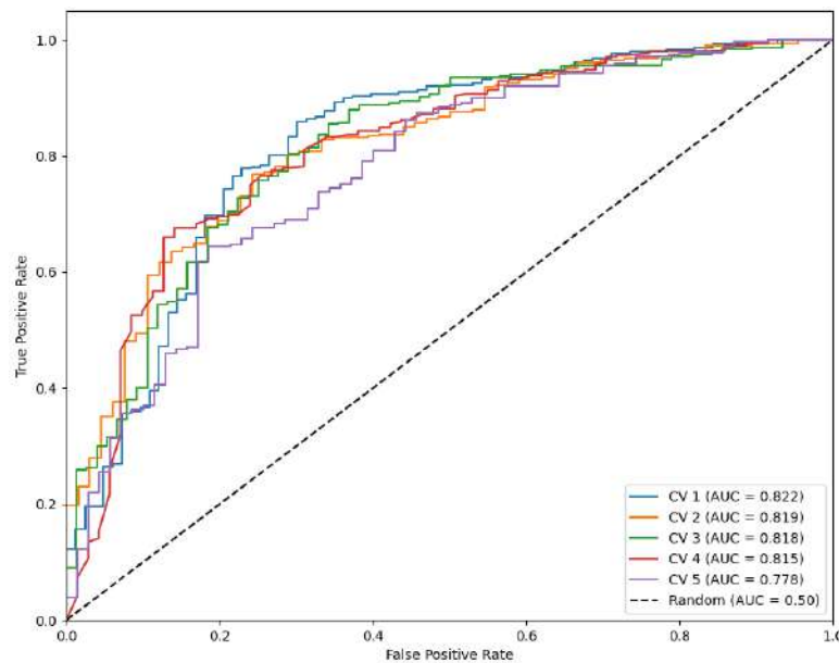
Figure 2. ROC Curves with normal data
