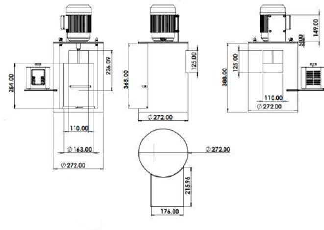
Figure 1: projection drawing of the mixer
