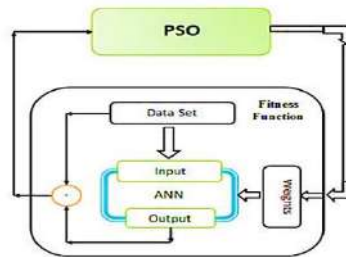
Figure 1: ANN training using PSO (Matrood and Sedeeq, 2020)
