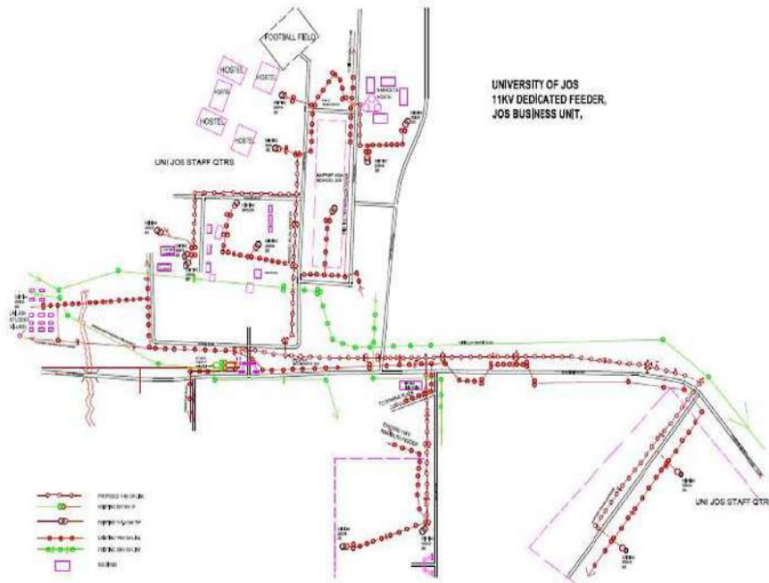
Figure 1. A sketch of the 11 Kv dedicated Feeder of the University of Jos.
