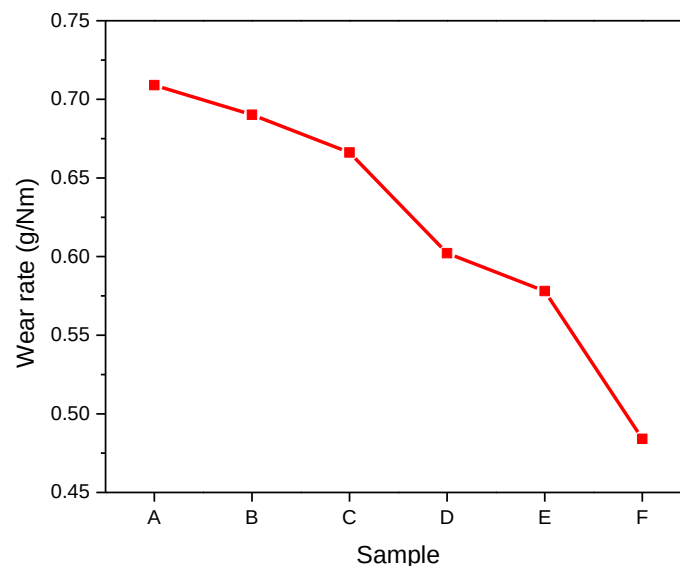
Figure 6: Results of the wear rate
