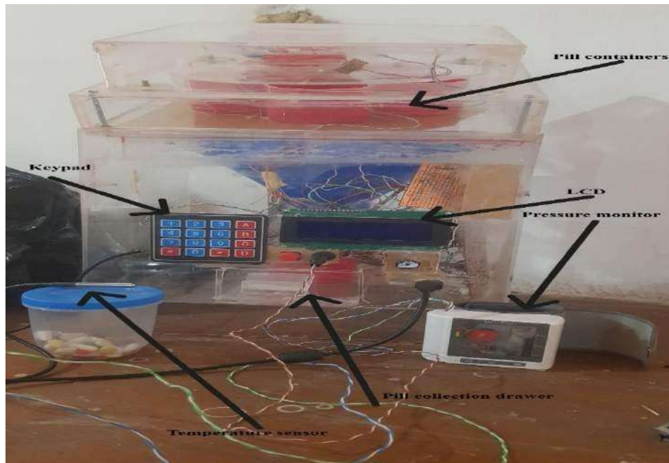
Fig 7 Developed system
