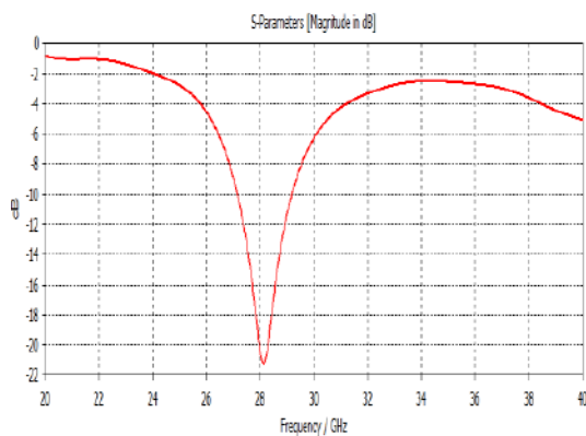
Figure 2: Return loss plot
