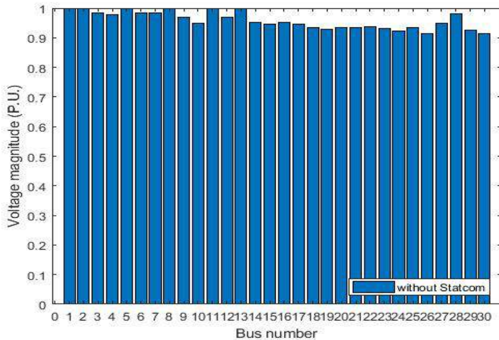
Figure 5: Voltage Profile of the network without STATCOM
