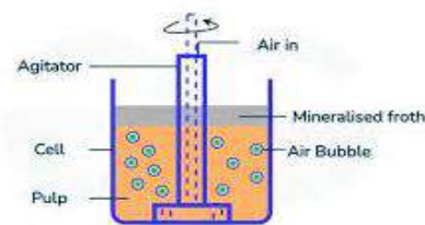
Figure 1: Froth flotation process
