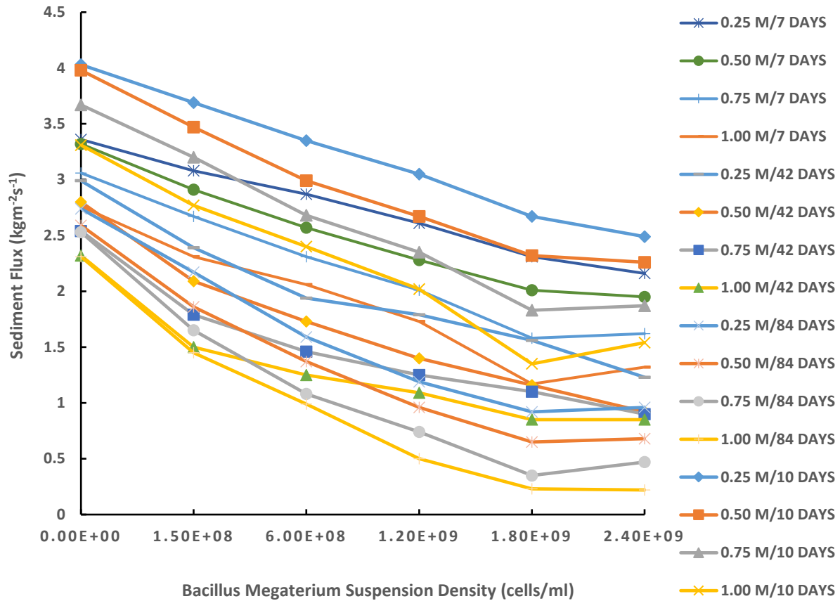
Figure 4: Variation of sediment flux of soil-cementation reagent mixture with B. megaterium suspension density at 14 \text{ ms}^{-1} speed for 7, 42, 84 days of curing and 3 days of soaking.
