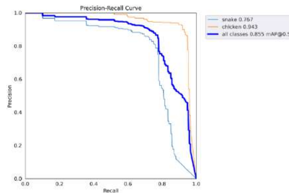
Figure 10: Precision-Recall Curve
