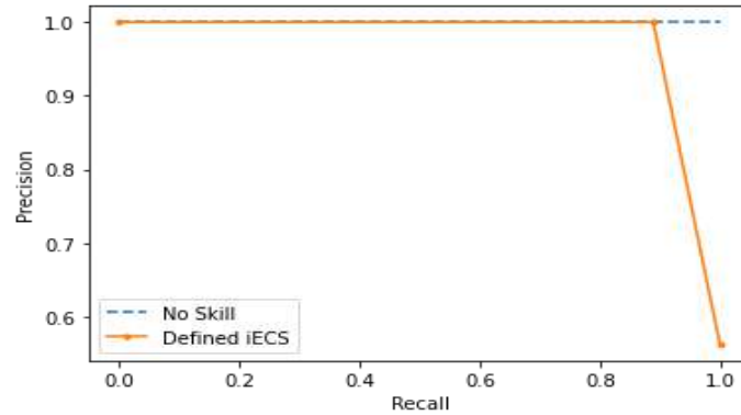
Figure 6: Precision-Recall curve
