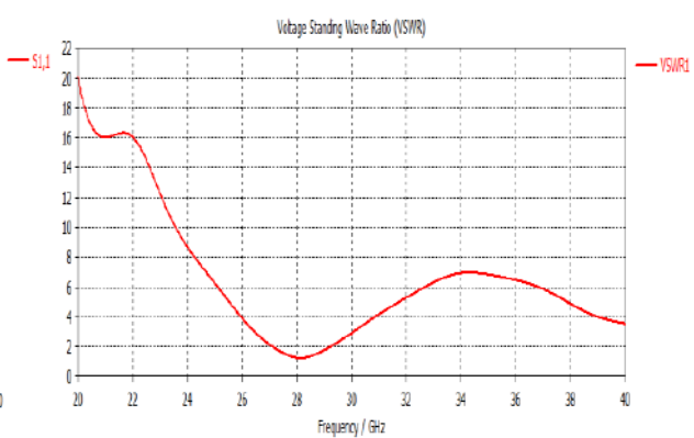
Figure 3: voltage standing wave ratio
