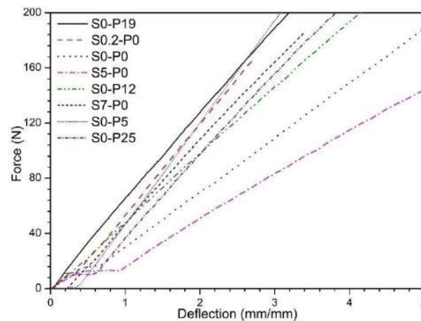
Figure 7: Force-Deflection curve for single-phase reinforcement of polyester/sugarcane bagasse/ plantain peel composite
