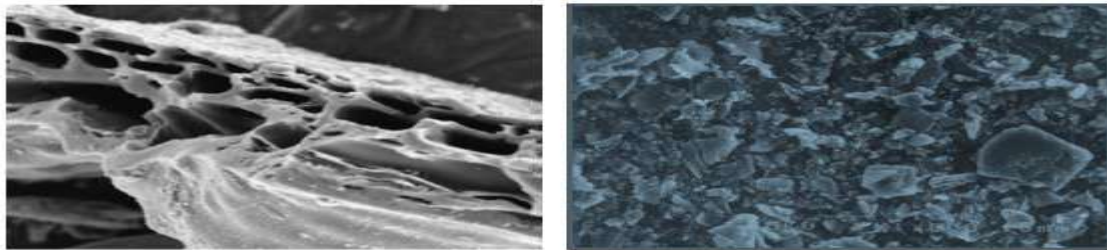
Figure 2: Scanning Electron Microscopy analysis of Greek and Pakistan Rice Husk Ash (RHA)
