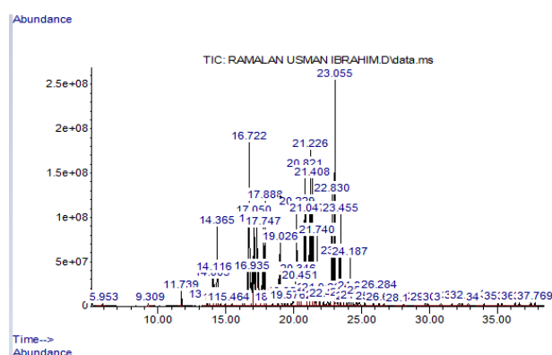
Figure 6: GC-MS spectrum of Roselle brake fluid
