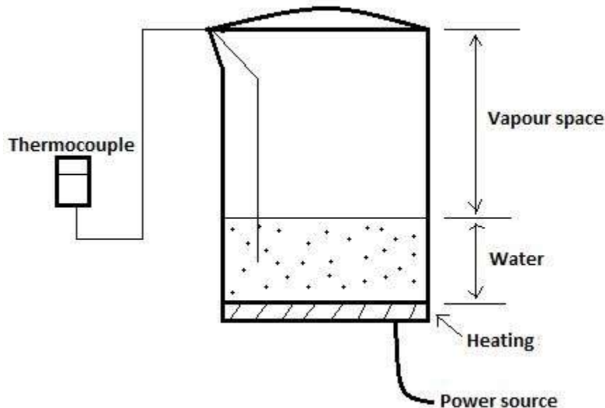
Figure 1. Experimental setup
