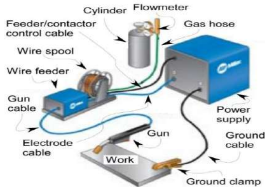
Plate 2: Gas metal arc welding (GMAW) process (source: [12]).
