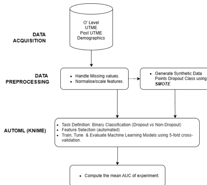
Figure 1. Schematic of the flow of AutoML Experiment.
