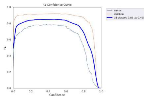
Figure 9: F1_score-Confidence curve
