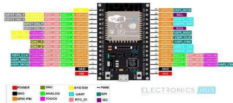
Fig 3 ESP32 microcontroller (Rishit, 2019)
