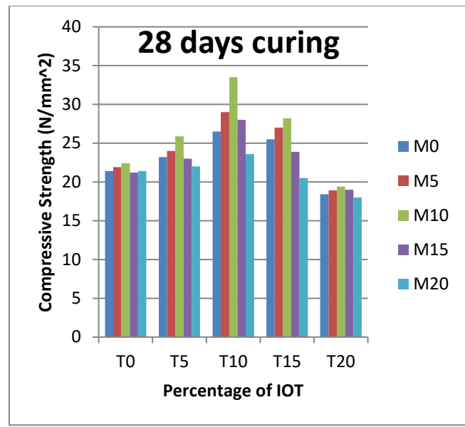
Fig 2: Compressive Strength of MK-IOT blends at 28 days curing
