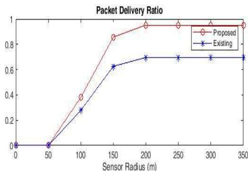
Fig. 5 packet delivery ratio for 60 nodes
