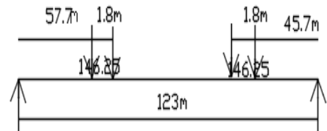
Fig. 2: Statical Diagram for Maximum Moment and Shear.
