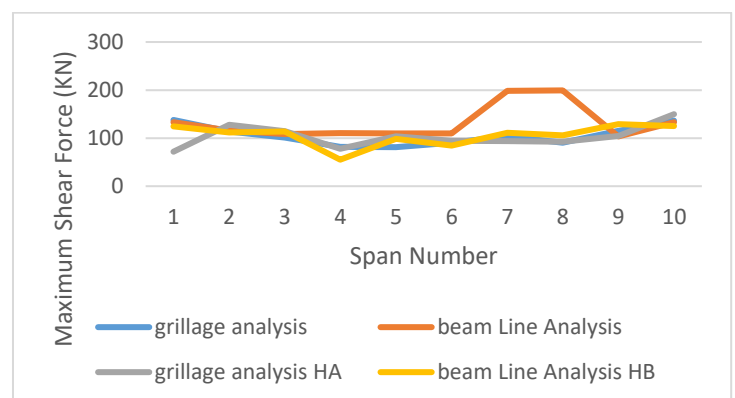
Fig. 5: Maximum Shear Force Comparison for HA and HB loading
