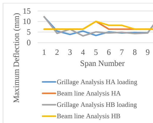
Fig. 6: Deflection Comparison for HA and HB Loading
