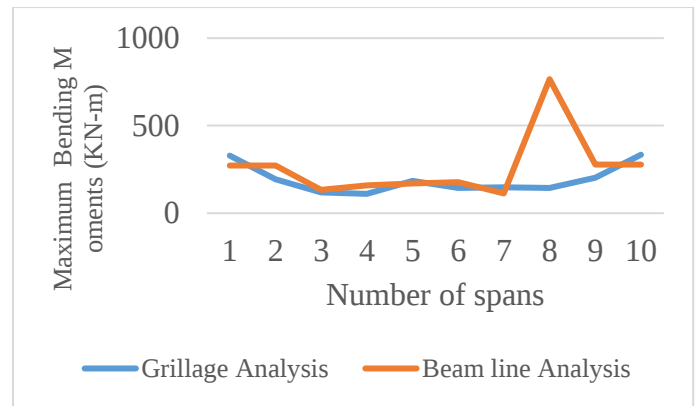
Fig. 4b: Bending Moments comparison for Maximum Span Moments for HB loading
