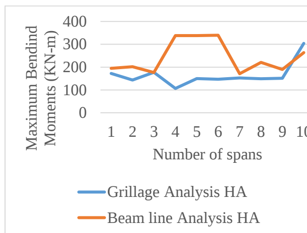
Fig. 4a: Bending Moments for Maximum Span Moments for HA loading
