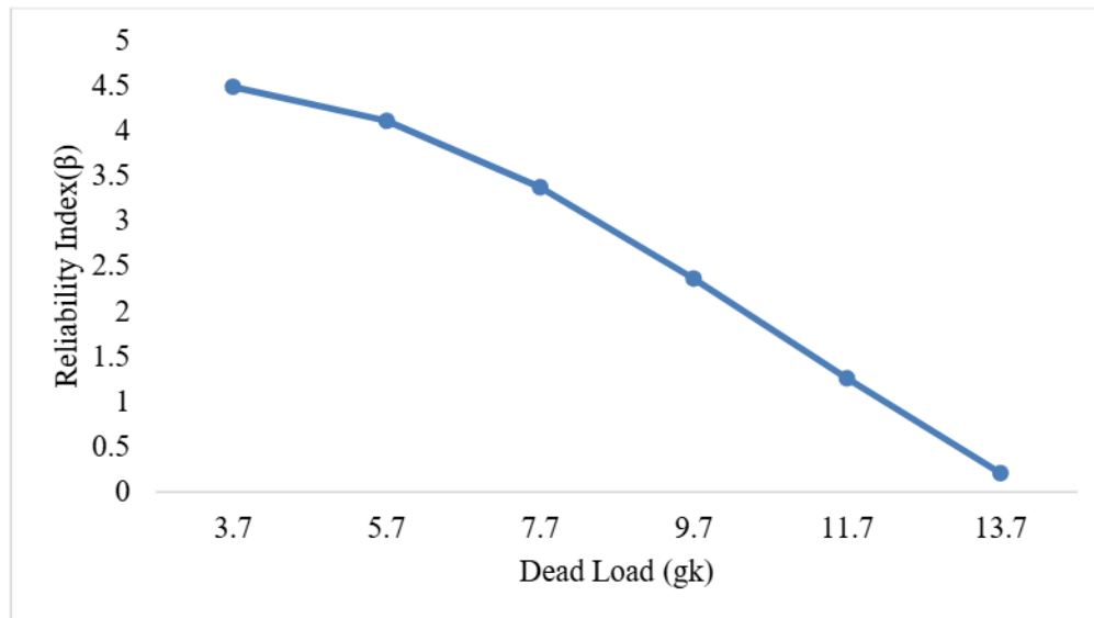
Fig. 5.: Relationship between dead load and reliability index in bending
