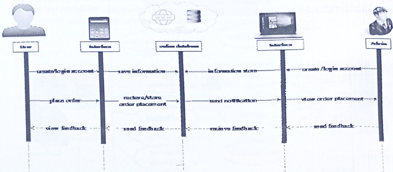
Figure 3: The Proposed Systems' Sequence Diagram
