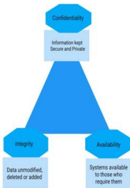
Fig 1: CIA Principles
