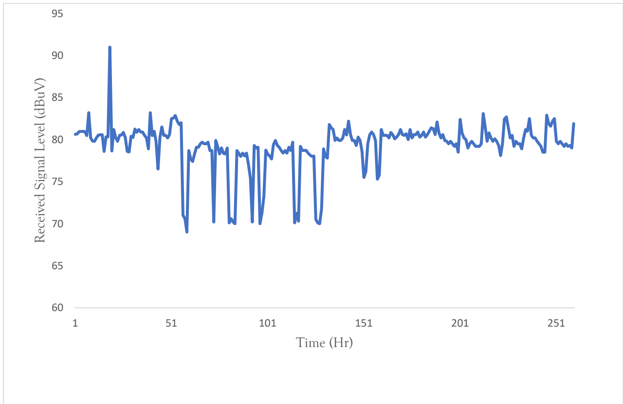
Figure 5: Measured real-time digital television signals
