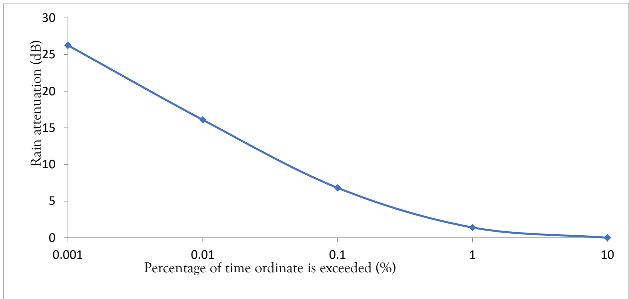
Figure 3: Rain attenuation's cumulative distribution at Ku-band, 42.5°
