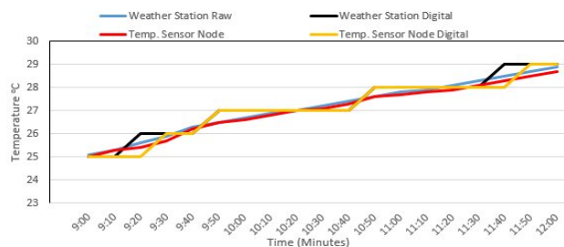
Figure 6. Comparison of Reference and the Developed Sensor Node Temperature Data.
