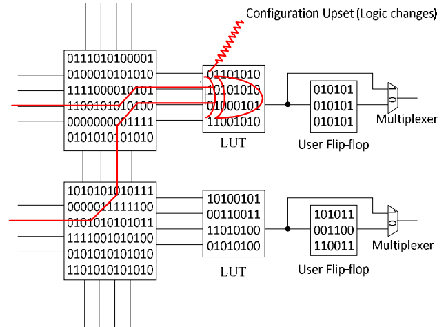
Figure 3: Upset in Logic [19].
