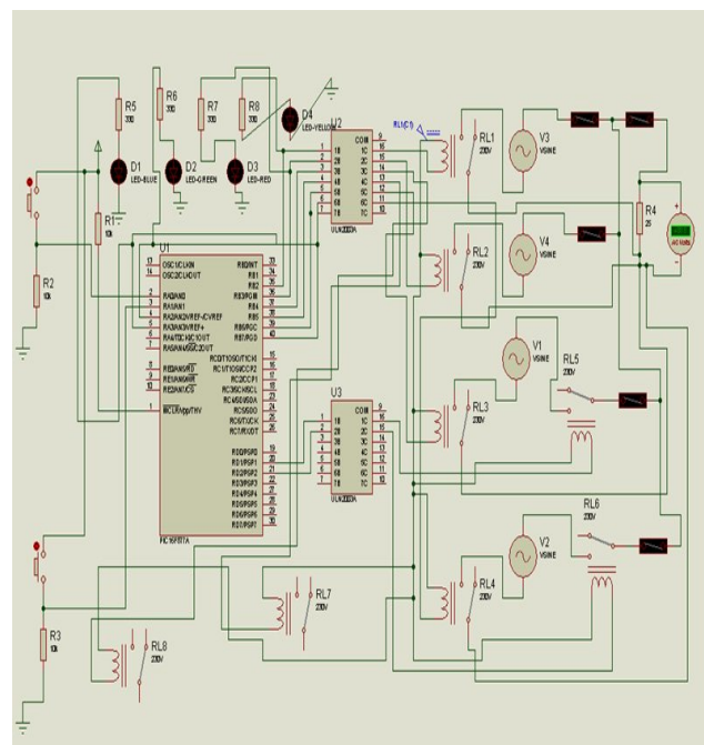
Figure 2: Simulation Circuit
