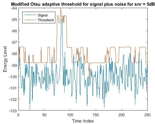
Figure 4: Detection thresholds for MO-CFAR algorithm for signal to noise ratio of 5dB.
