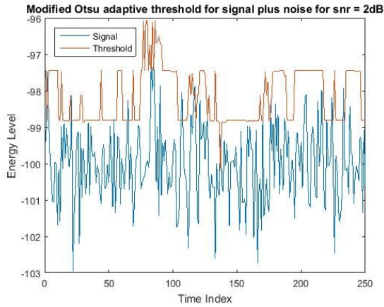
Figure 3: Detection thresholds for MO-CFAR algorithm for signal to noise ratio of 2dB.
