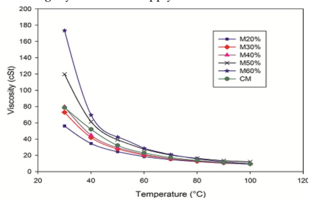
Figure 1. Viscosity-temperature plots of the mixed
