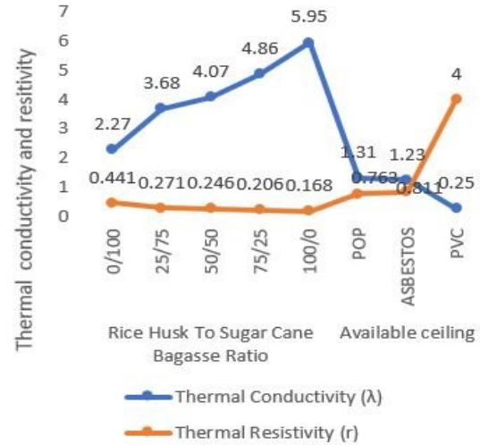
Figure 1: Thermal conductivity and resistivity test result from the composite and available ceiling
