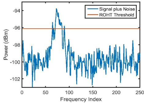
Figure 7: Signal plus Noise spectra at SNR = 5 dB showing the threshold estimated by the ROHT algorithm
