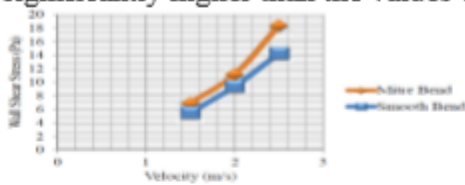
Figure9: Graph of Wall Shear Stress against Fluid Flow Velocity
