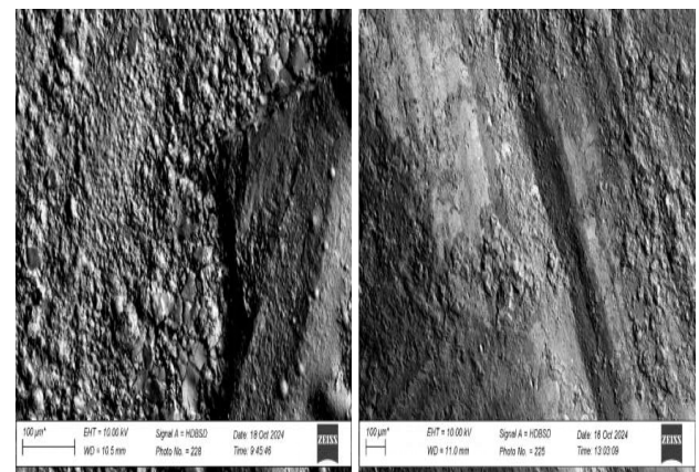
Figure 5: Microstructure of GRA-optimised (a) FCA (b) MIG weldment at 100 \mu\text{m} scale
