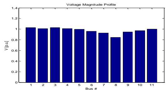
Figure 2: Voltage profile of the case study network without PDC and STATCOM
