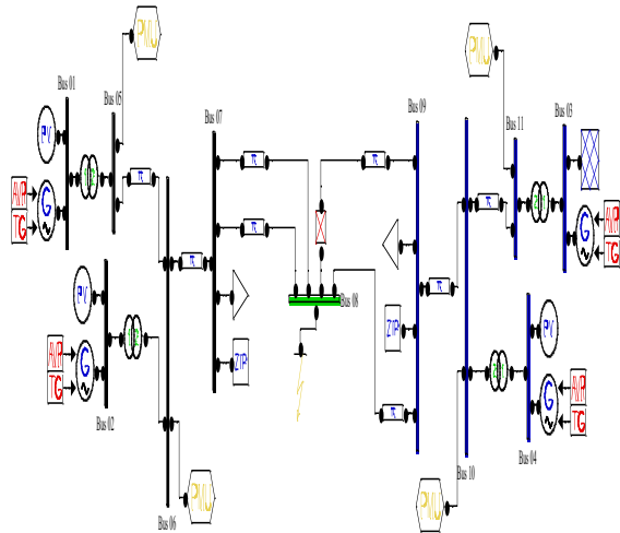
Figure 1: Kundur four machine 11 bus two area power system.
