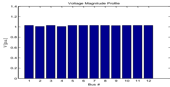
Figure 3: Voltage profile of the case study network modified with PDC and STATCOM
