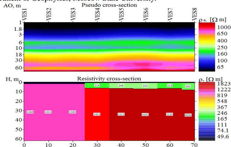
Fig.3 (a) Pseudo cross-section and 3(b) Resistivity cross-section of VES 1-8 along profile A in AnguwanJukpa.
