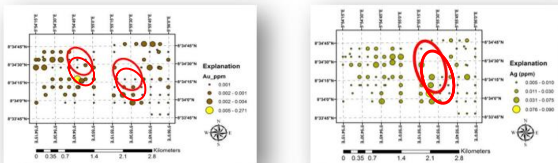
Figures 12: Concentration Point Map of Gold and Silver in the Residual Soil of the Study Area
