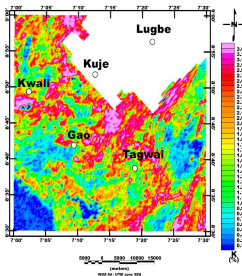
Figure 9. Potassium concentration map
