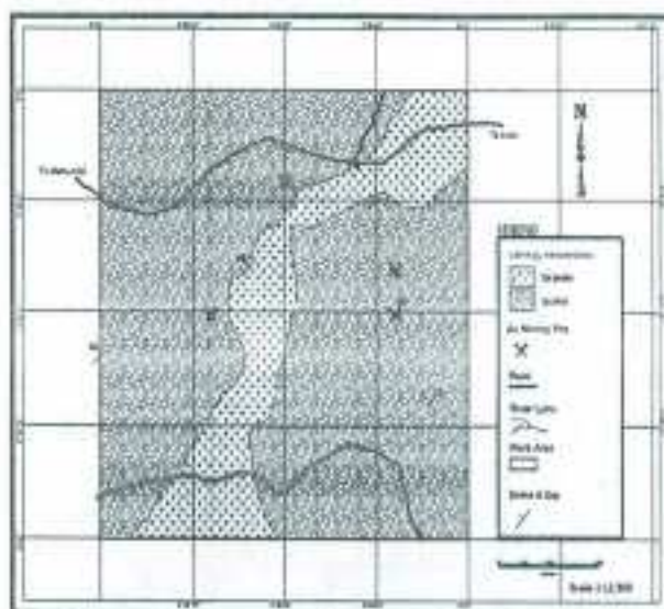
Figure 1: Geological Map of Luku.
