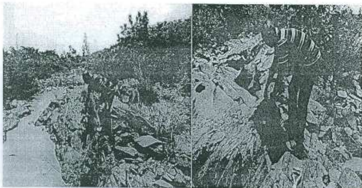
Figure 2. Shows photograph of schist being the dominant rock in the study area. They are generally low-lying, light coloured with characteristic medium to coarse grained texture. Mineral components of the rock consist of quartz, feldspar and mica. The schist is slightly weathered and foliated. The rock generally trend in NW-SE direction and generally dips between 30^{\circ} - 40^{\circ} NW. These rocks are jointed and the joints are filled with quartz vein.
