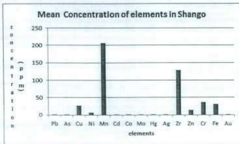
Figure7. mean concentration of elements in the soils in Shango area
