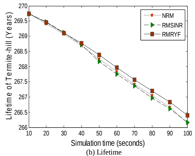
Figure 3: Energy efficiency and Lifetime comparison of Termite-hill routing algorithm for different radio models (NRM, RMSINR and RMRYF).
