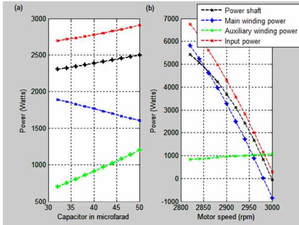
Figure 5. Power-capacitor and Power-motor speed characteristics
