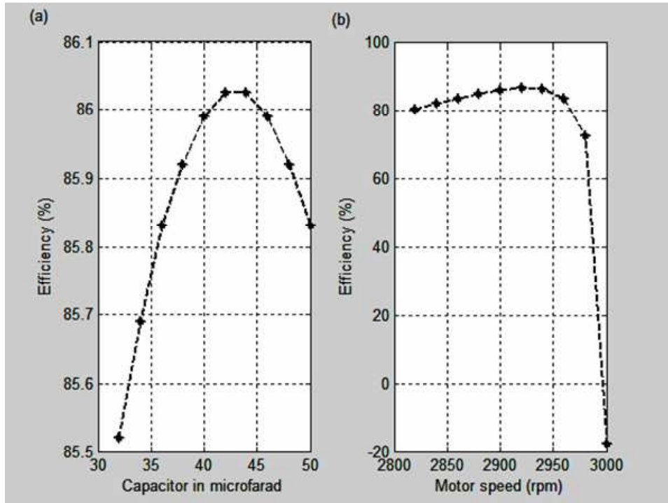
Figure 2. a) Efficiency-capacitor and b) Efficiency-Motor speed characteristics
