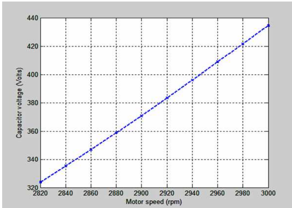
Figure 6. Capacitor voltage-motor speed characteristic
