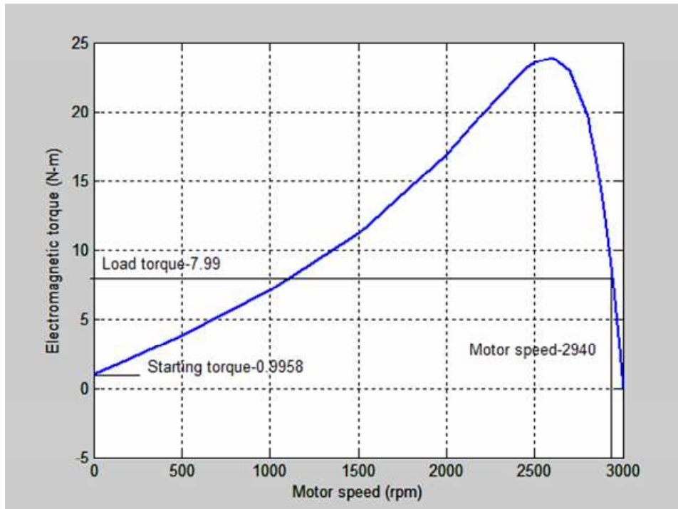
Figure 8. Mechanical torque-rotor speed characteristic
