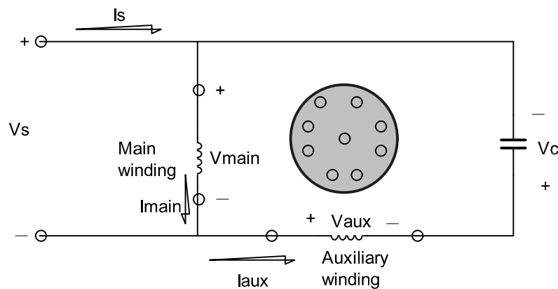
Figure 1. Permanent split capacitor ac induction motor circuit
