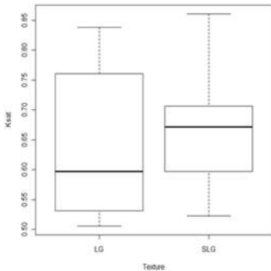
Figure 7. Boxplot of Ksat by texture class
