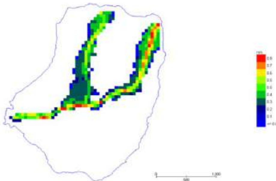
Figure 11. This shows clearly that the basal friction which is a function of the coefficient of friction (manning's, n) is one of the main components of debris flow dynamics. It tends to reduce or slow the flow of debris
