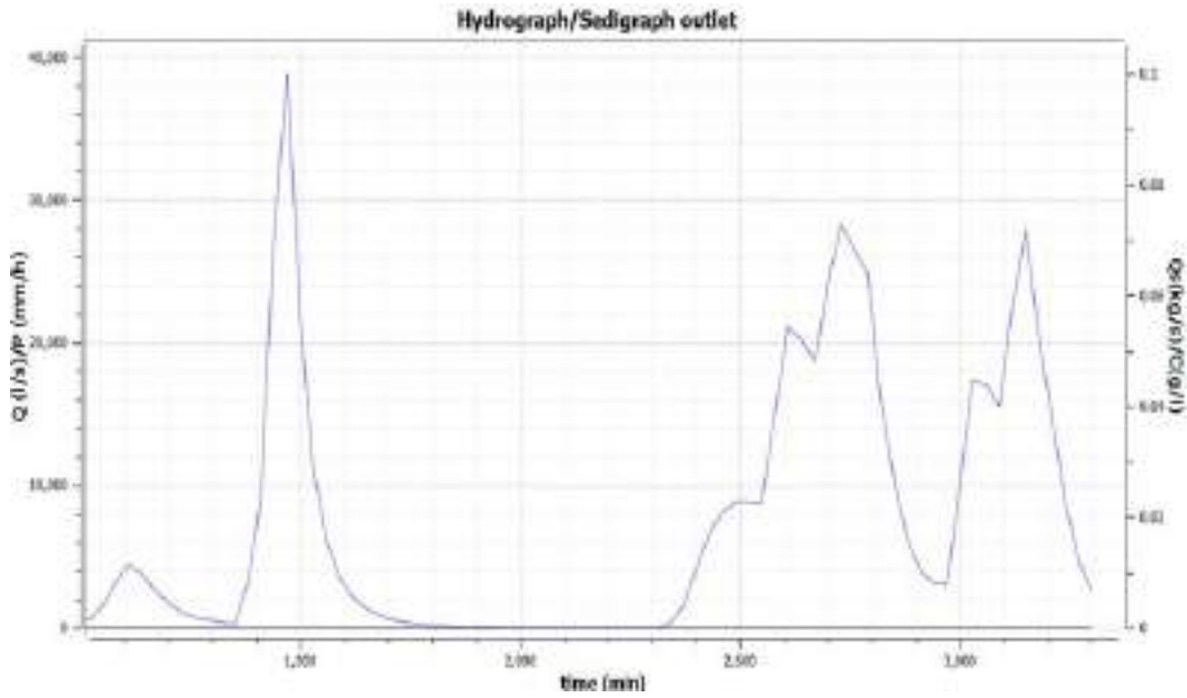
Figure 9. LISEM hydrograph
