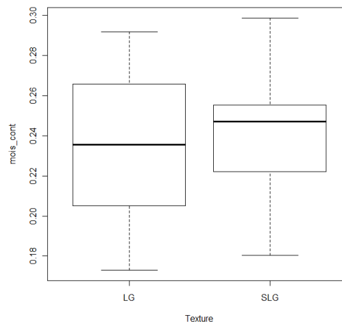
Figure 9. Moisture content by texture
