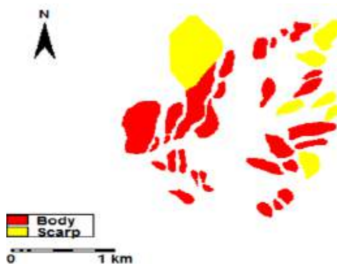
Figure 4. Landslides scarp and body as mapped in the field
