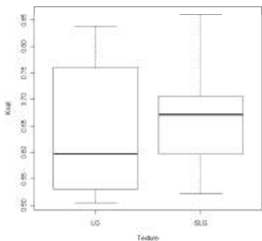
Figure 6. Ksat by texture class
