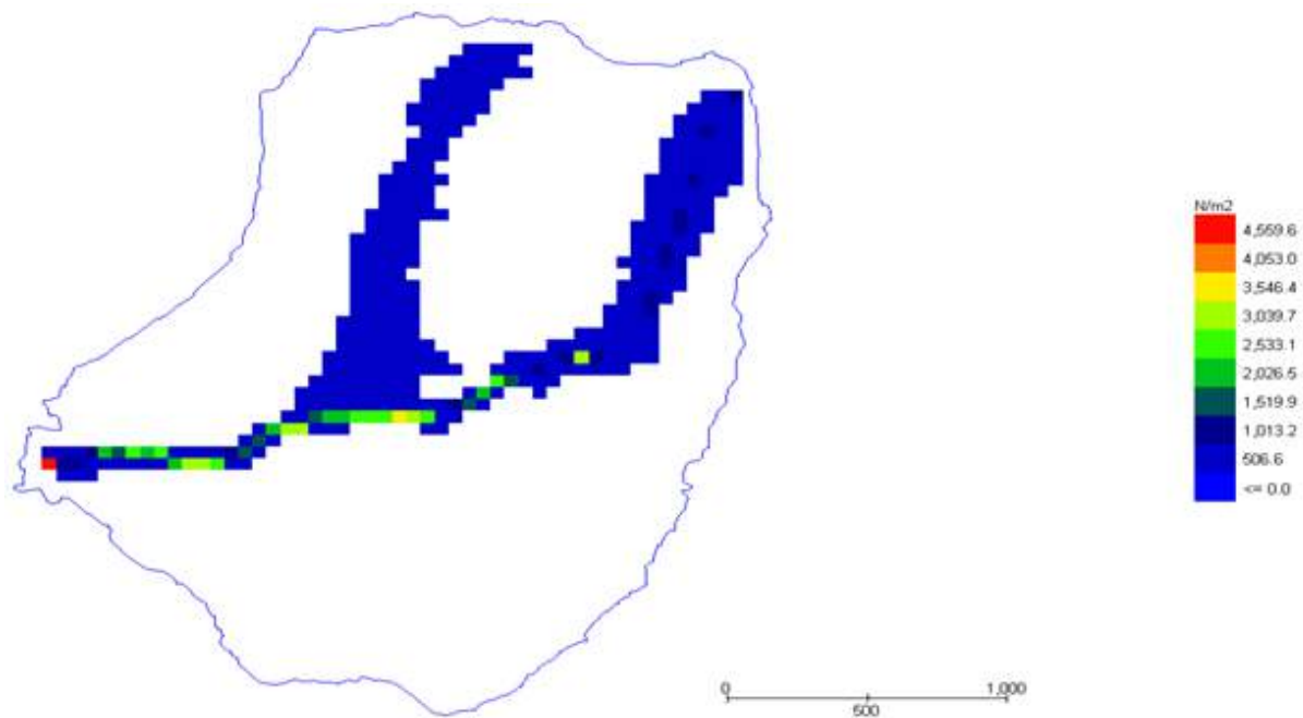
Figure 12. Debris flow grid impact force
