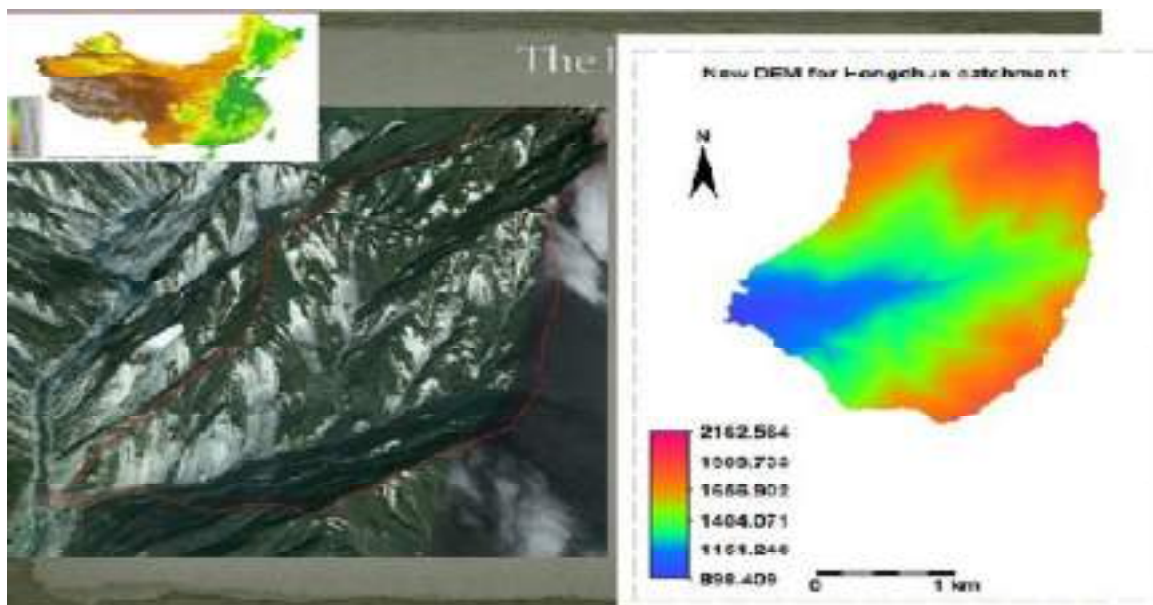
Figure 1. Yingxiu catchment and digital elevation model of the study area
