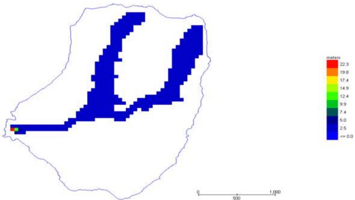
Figure 11. Debris flow grid maximum depth
