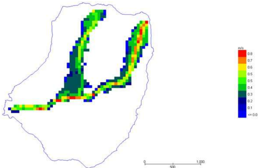
Figure 13. Debris flow grid maximum velocity
