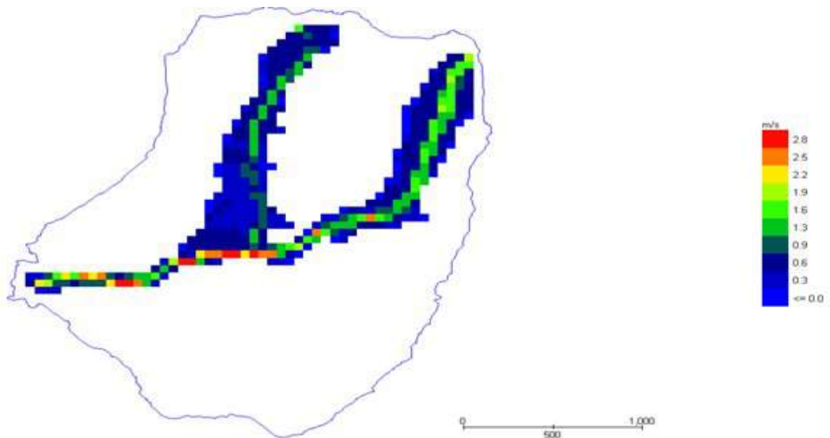
Figure 10. Debris flow grid maximum velocity
