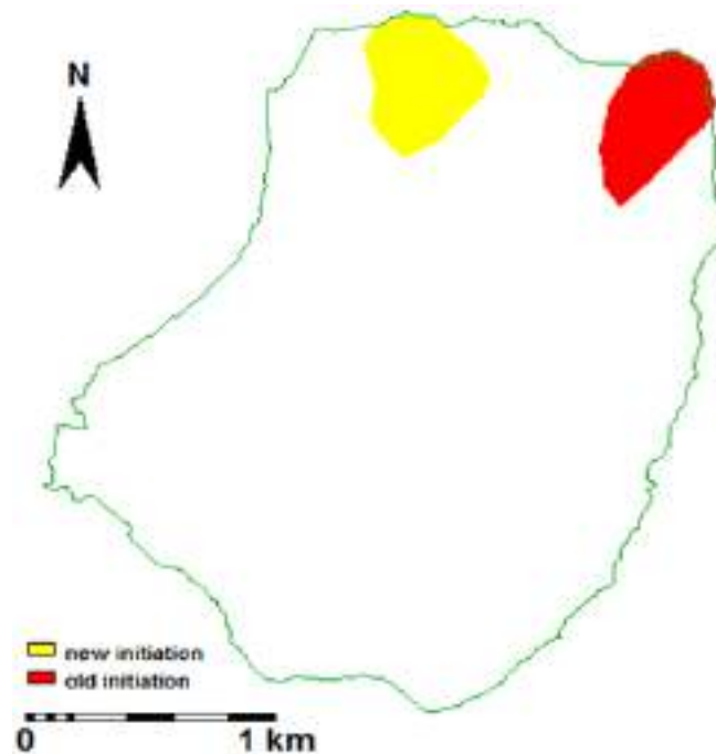
Figure 5. diagram showing debris flow initiation areas of the landslides
