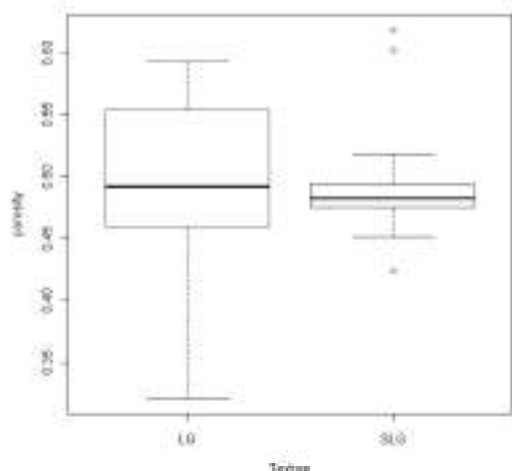
Figure 8. Porosity by texture class
