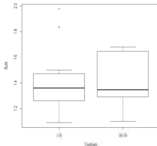
Figure 7. Box plot of Bulk density by texture class
