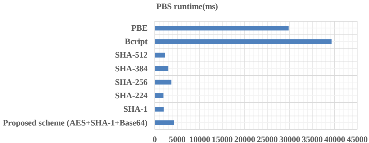
Figure 2: PBS runtime compared outputs.
