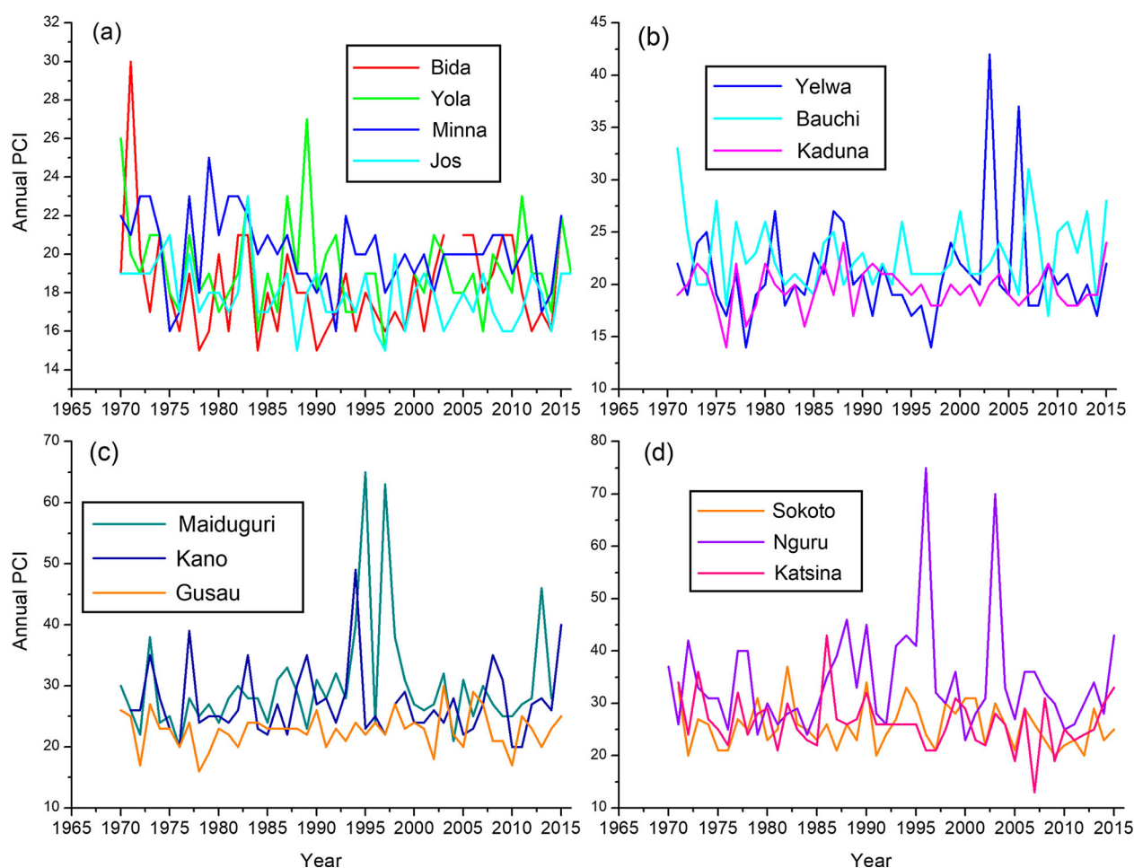
Fig. 2 Precipitation concentration index series for (a) Bida, Yola, Minna, and Jos; (b) Yelwa, Bauchi, and Kaduna; (c) Maiduguri, Kano, and Gusau; and (d) Sokoto, Nguru, and Katsina.
