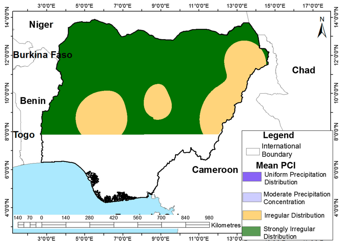
Fig. 3 Mean annual precipitation concentration index.
