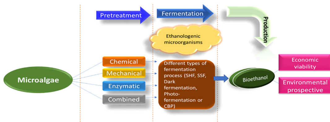
FIGURE 14.3 Adapted: A general outline of the different pretreatment and fermentation methods involved in the synthesis of bioethanol from microalgae (Phwan et al., 2018). Source: Extracted from Phwan, C.K., Ong, H.C., Chen, W.-H., Ling, T.C., Ng, E.P., Show, P.L., 2018. Overview: comparison of pretreatment technologies and fermentation processes of bioethanol from microalgae. Energy Conversion and Management , 173, 81–94.
