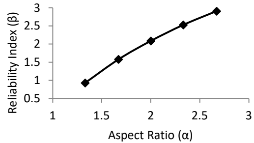
Fig. 2: Reliability Index-Aspect Ratio Relation for Nigerian Timber for Failure Mode 1
