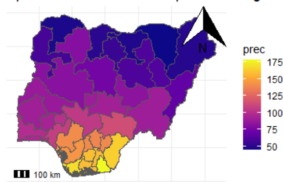
Spatial Distribution of Precipitation in Nigeria
