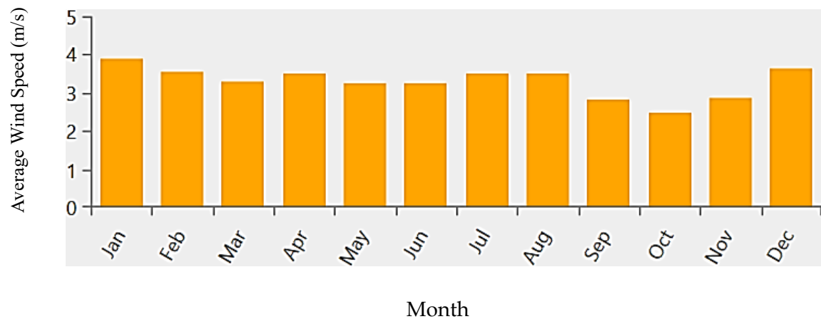
Figure 4: Yearly Mean Wind Profile
