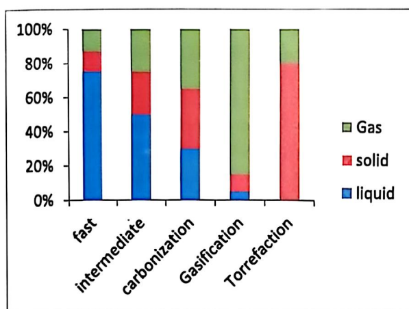
Figure 1: Mode of pyrolysis from wood biomass
