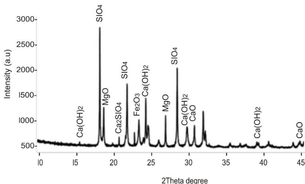
Fig. 10. Rice Husk Calcined at 800°C (KF)
