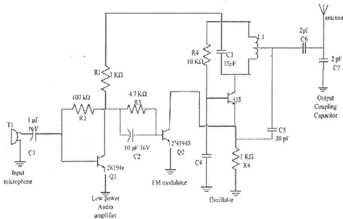
Fig 3.8 The Circuit Diagram Of The Radio Transmitter
