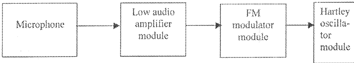
Fig. 3.2 Block Diagram Of The Radio Transmitter
