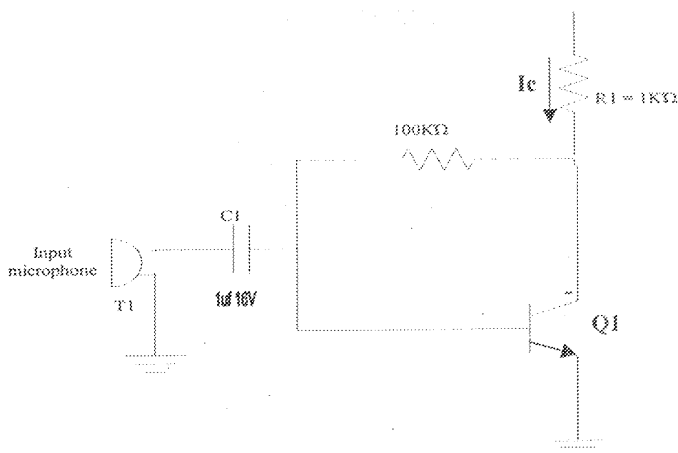
Fig 3.3 Low Power Audio Amplifier
