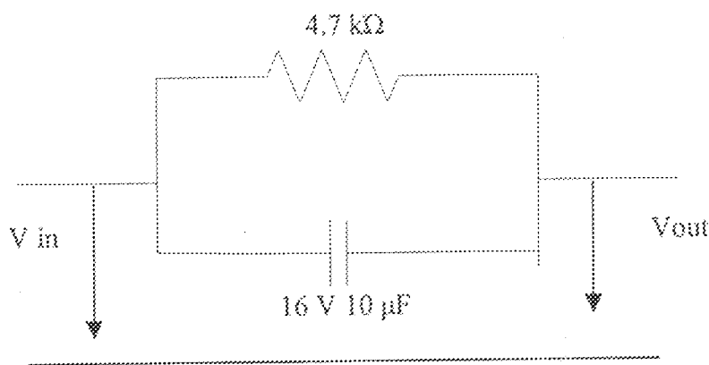
Fig 3.4 Pre-Emphasis Circuit
