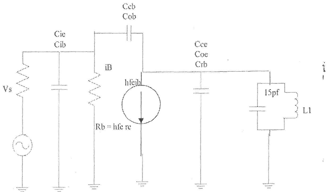
Fig 3.6 High Frequency Analysis Of A Common Base Amplifier
