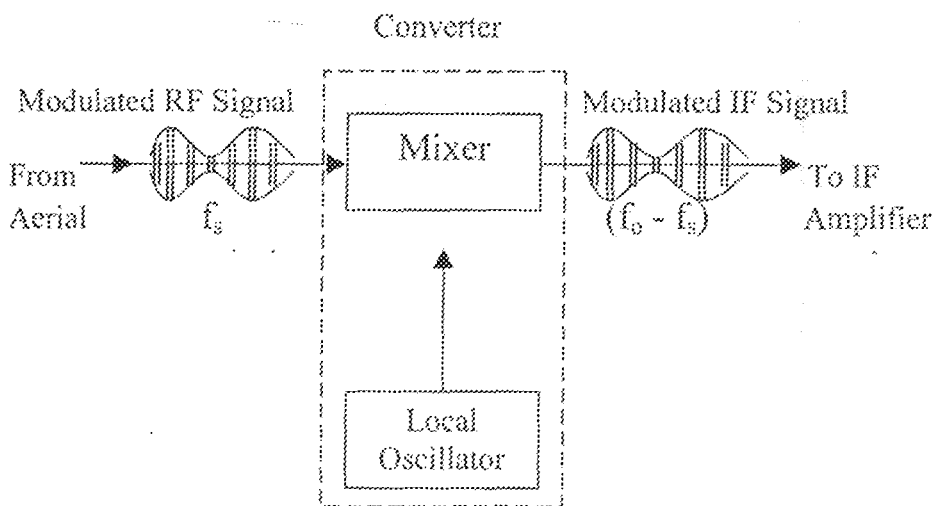
Fig 2.6 Frequency Conversion Module [1]
