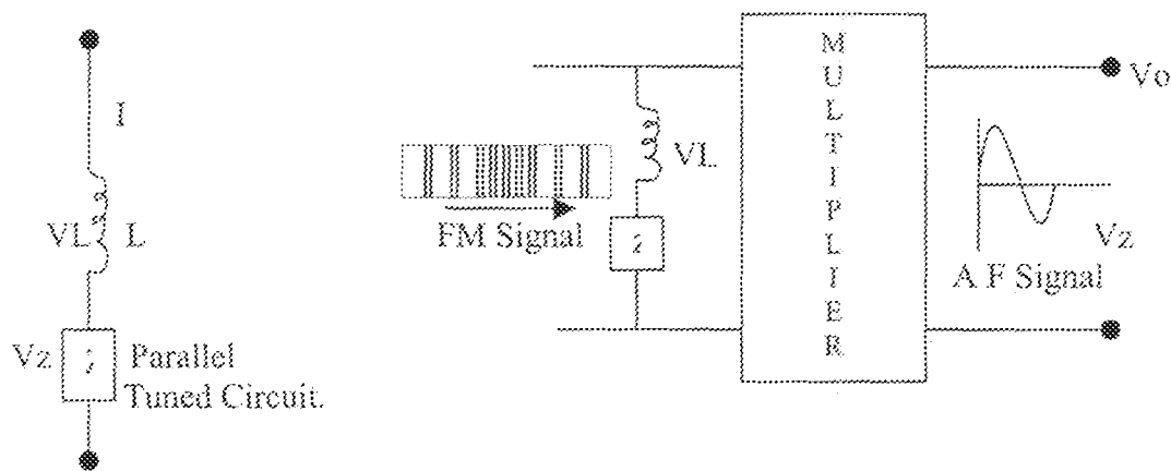
Fig 2.5 Multiplier Module [1]
