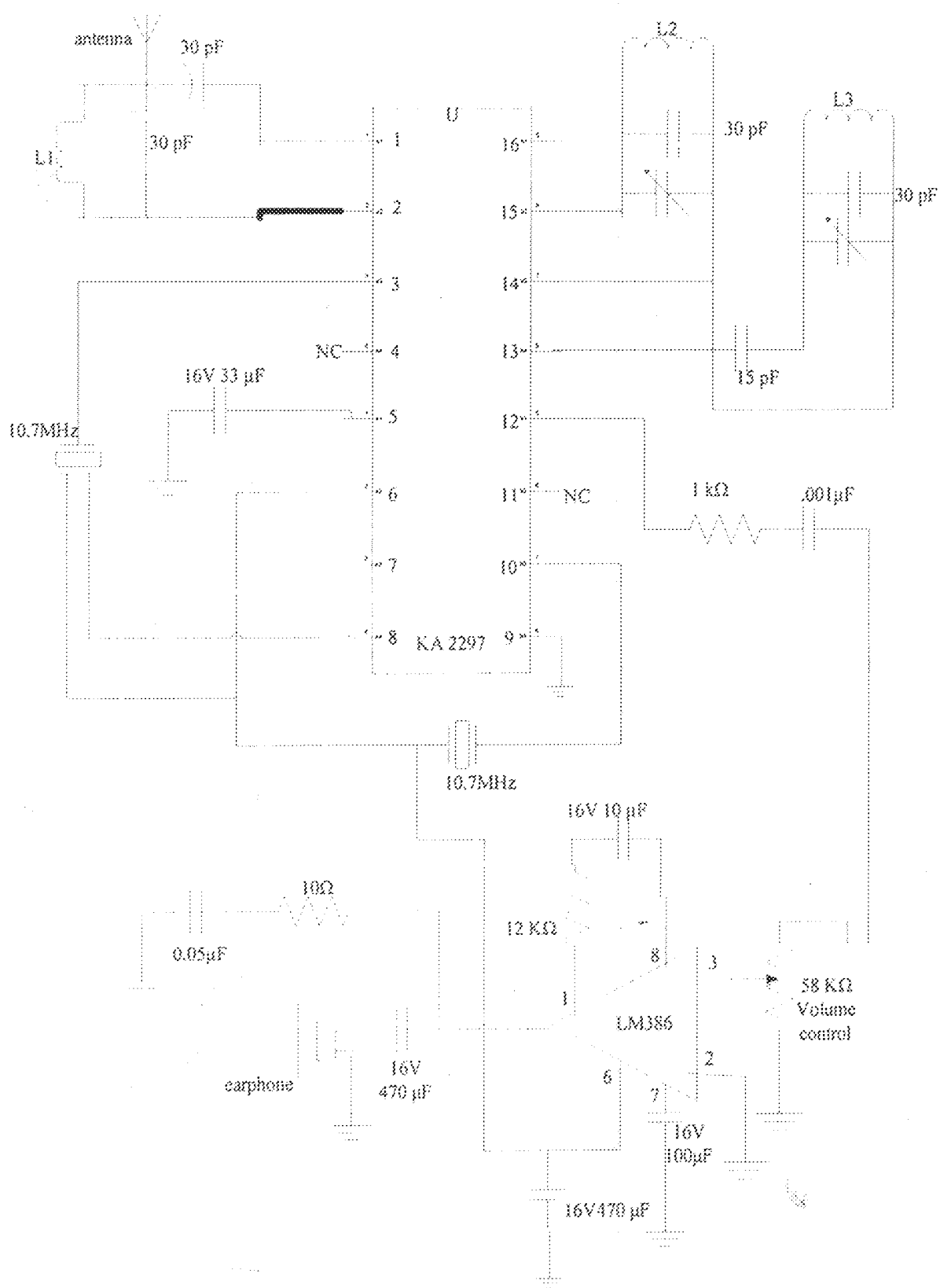
Fig 3.9 Receiver Circuit
