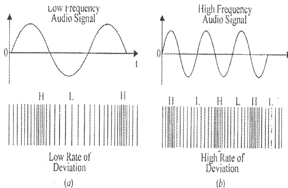
Fig 2.3 Rate Of Frequency Deviation [1]
