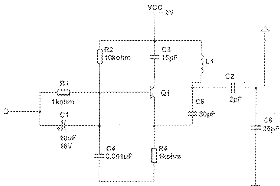
Fig.3.5 Fm Modulator Circuit
