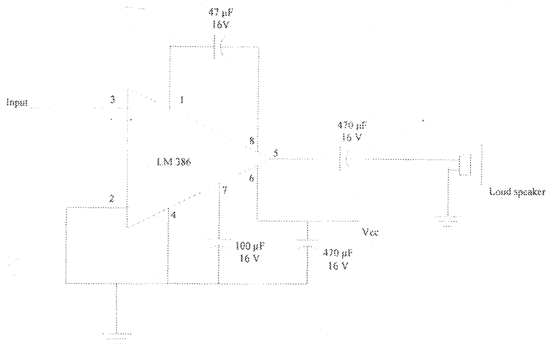
Fig 3.12 A Typical Circuit Of LM386
