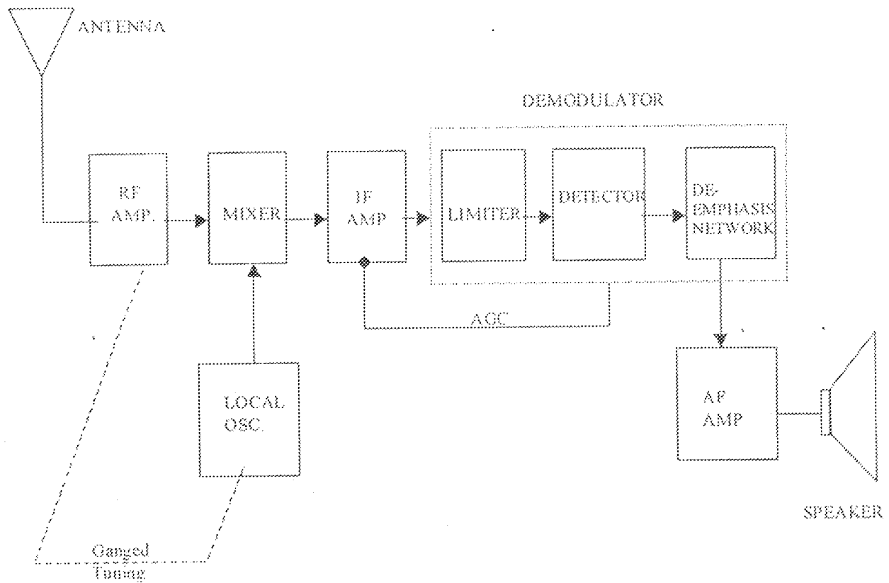
FIG. 2.6 BLOCK DIAGRAM OF AN FM RECEIVER
