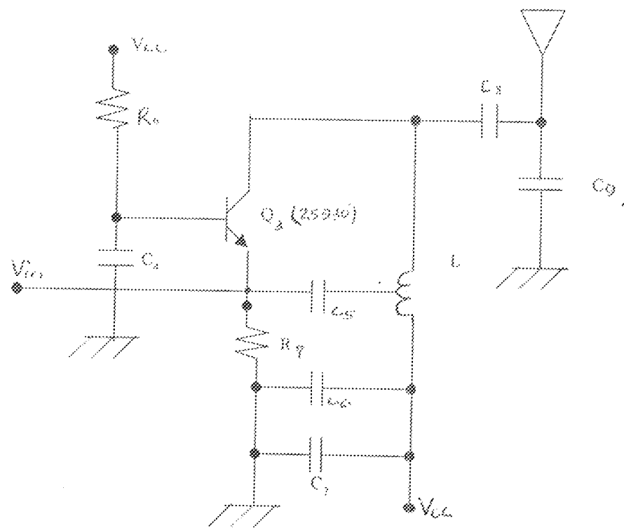
FIG.2.5 OSCILLATOR CIRCUIT/ANTENNA DIAGRAM
