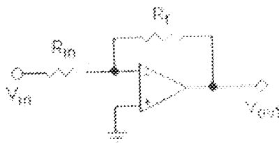
Fig. 2.9.2: Inverting amplifier configuration
