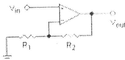
Fig. 2.9.1: Non-inverting amplifier configuration
