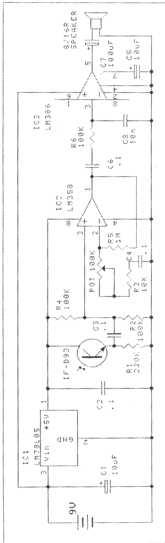
Fig.3.2.5: The One-way Fibre Optic Receiver Circuit
