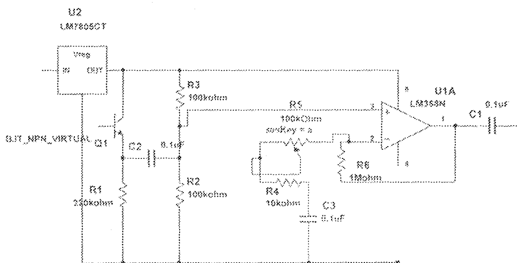
Fig. 3.2.2 Gain-determining circuit of the Rx
