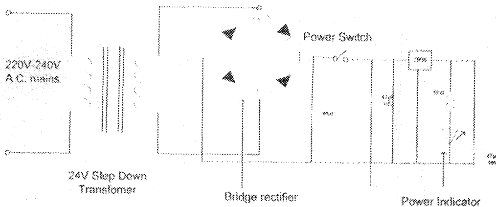
Fig.3.1 Power unit circuit [9]
