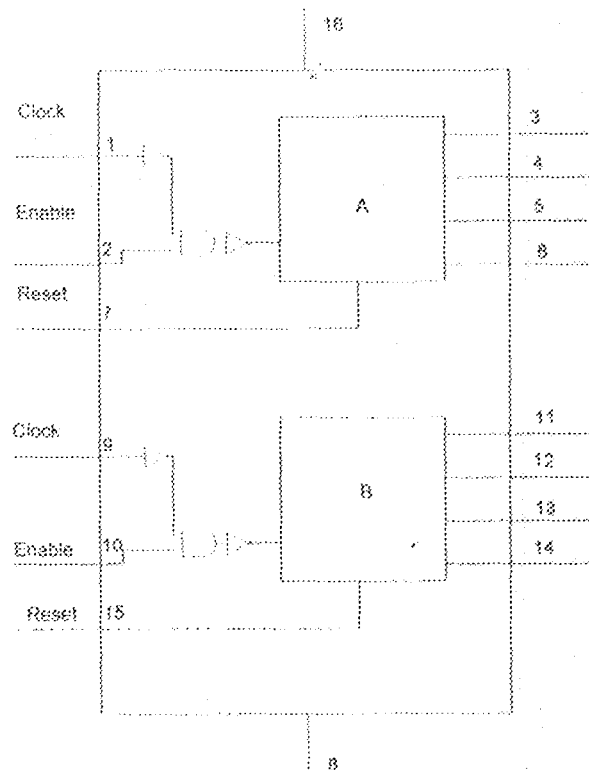
Fig. 3.9 functional diagram of the 4518B
