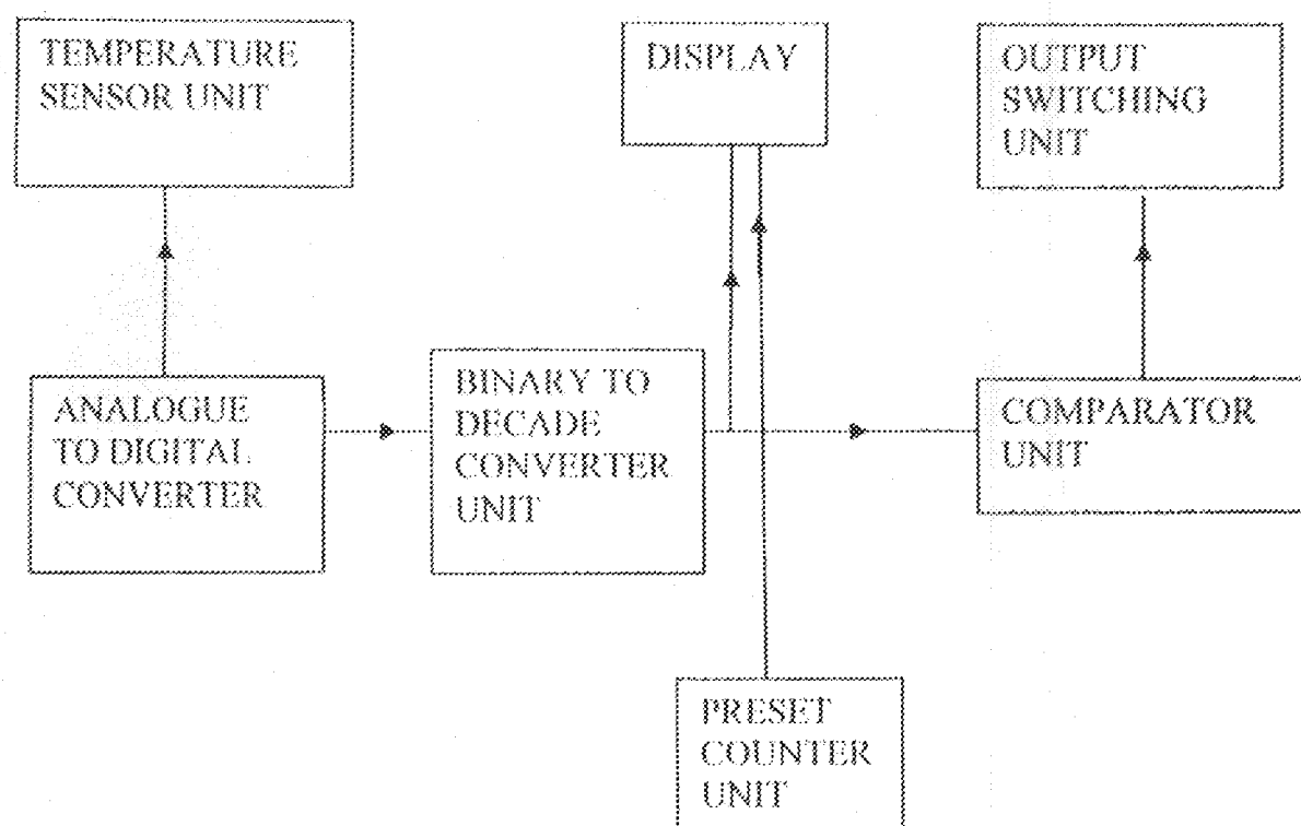
Fig. 1.1 Block Diagram
