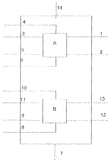
Fig. 3.13 The Pin Configuration of the 4013B
