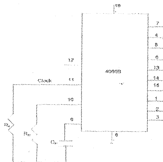
Fig. 3.14 The Functional diagram of the 4060B
