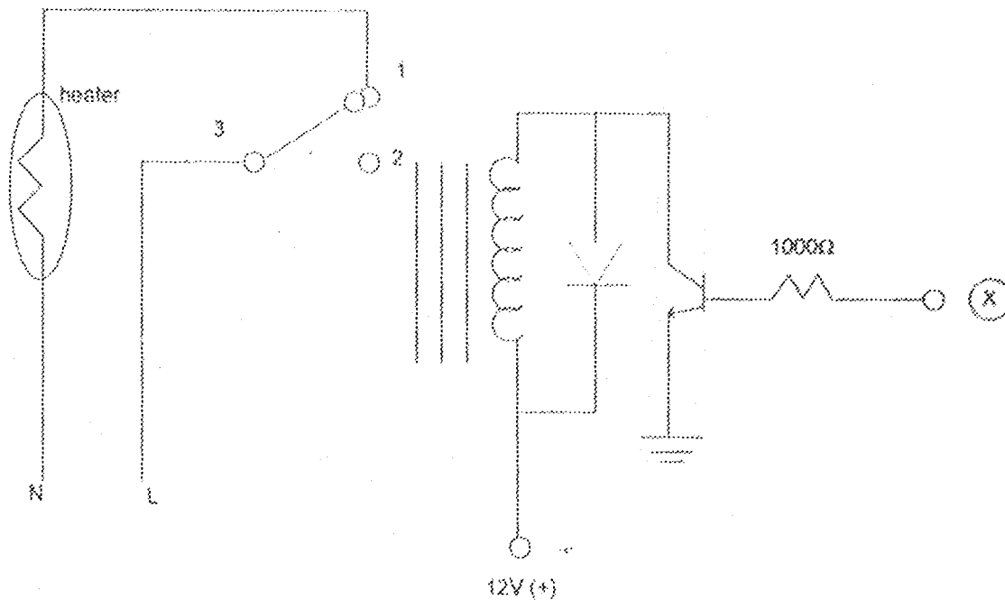
Fig. 3.16 the Output Switching Unit
