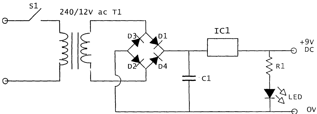
Fig 3.8 A complete power supply module
