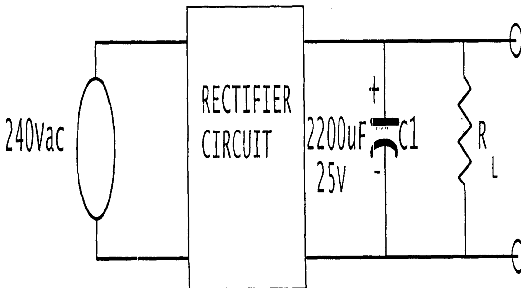
Fig 3.5 :( c) Shunt capacitor filter
