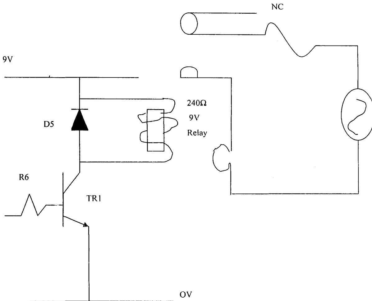
Fig 3.10 Schematic diagram of the switching module
