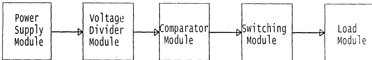
Fig 3.1 Block diagram of an automatic security outdoor lighting system.
