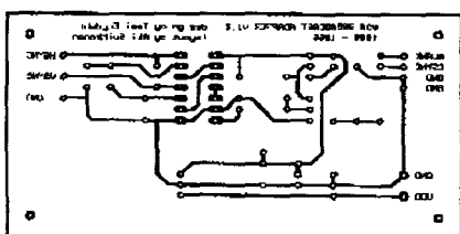
Fig 4.1 copper traces viewed from component side
