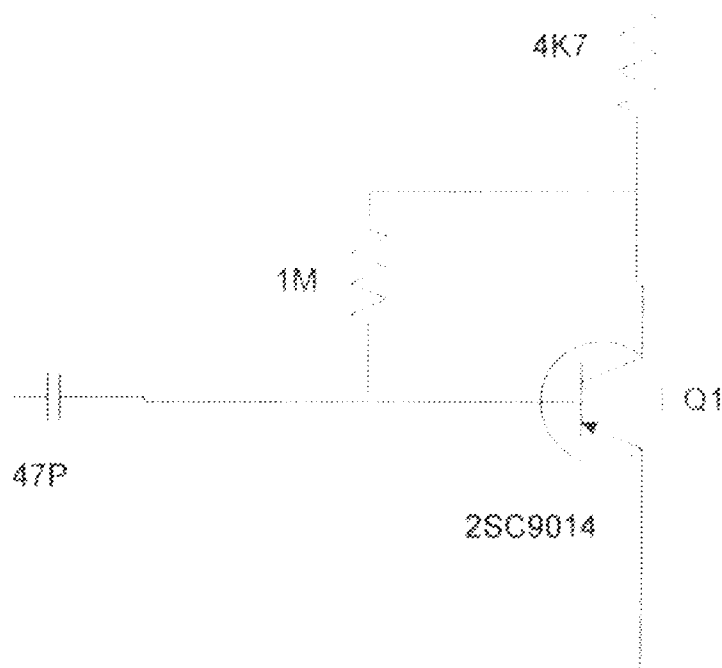
Fig 3.3 A radio Frequency Amplifier
