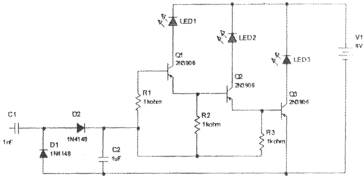
Fig 3.6 A transistor Stair Case
