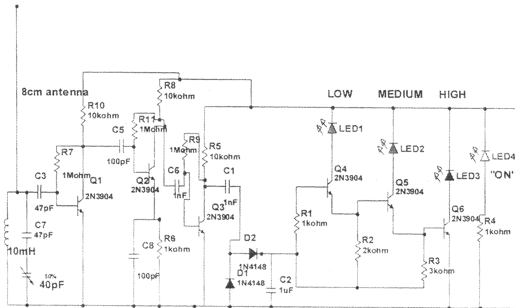
Fig 3.5 A generalized Circuit diagram of FSI
