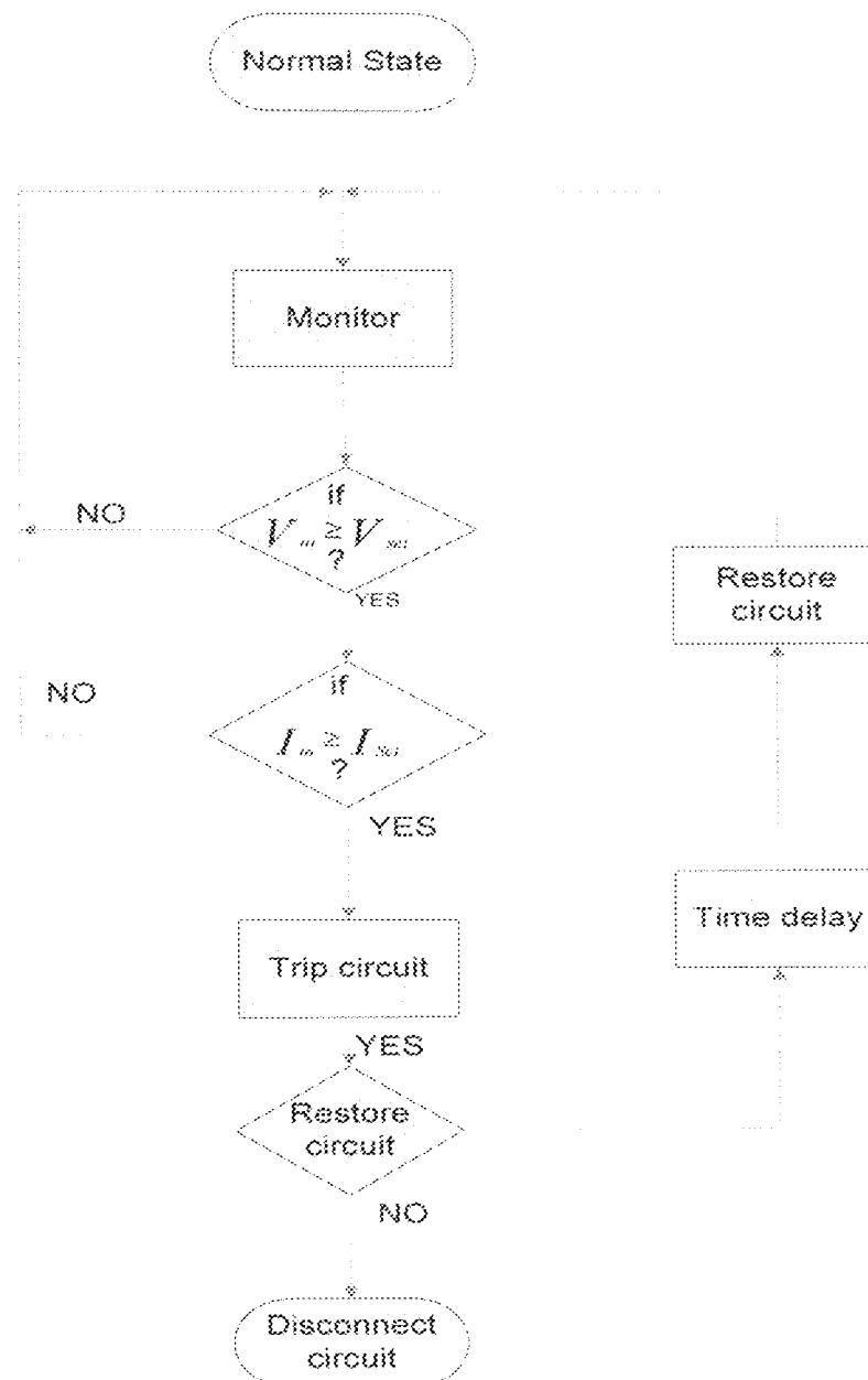
Fig 1.0 Flow Chart of Protective Device Functional Diagram
