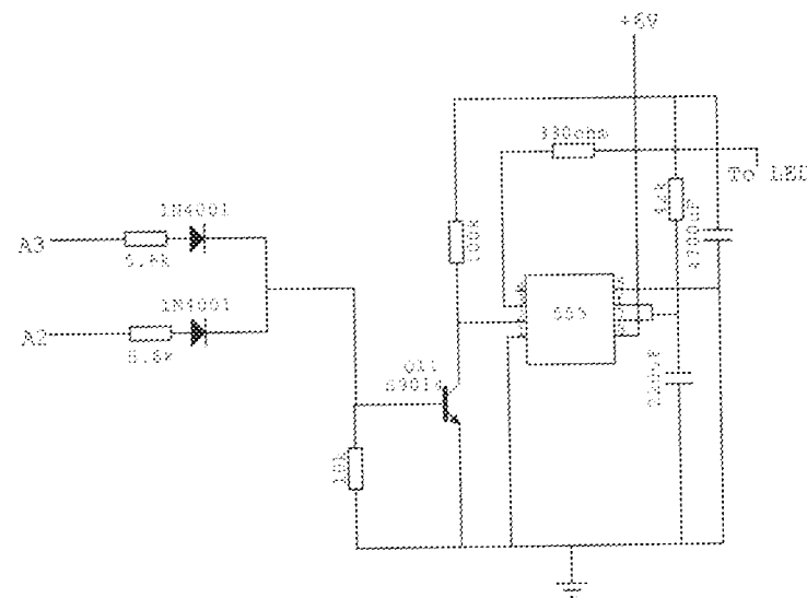
Fig. 3.5 10-Seconds Monostable Timeout Generator
