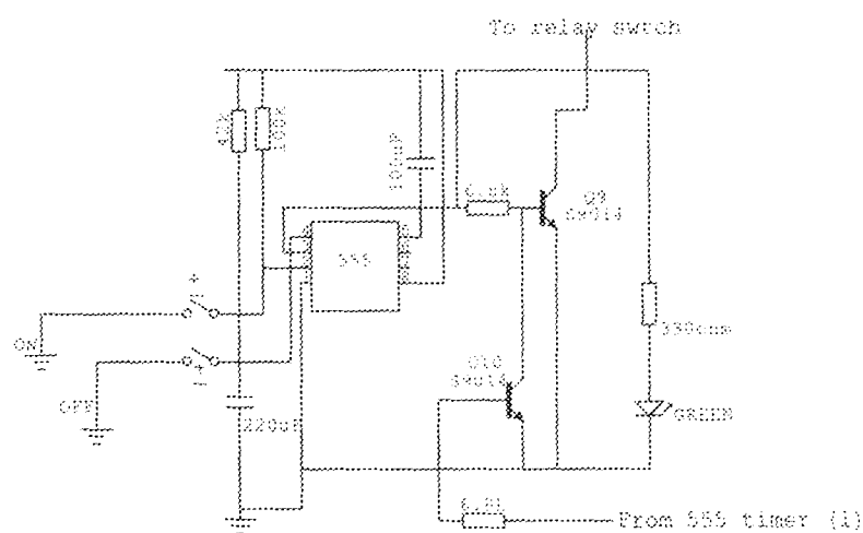
Fig. 3.7 On/Off Control of the circuit
