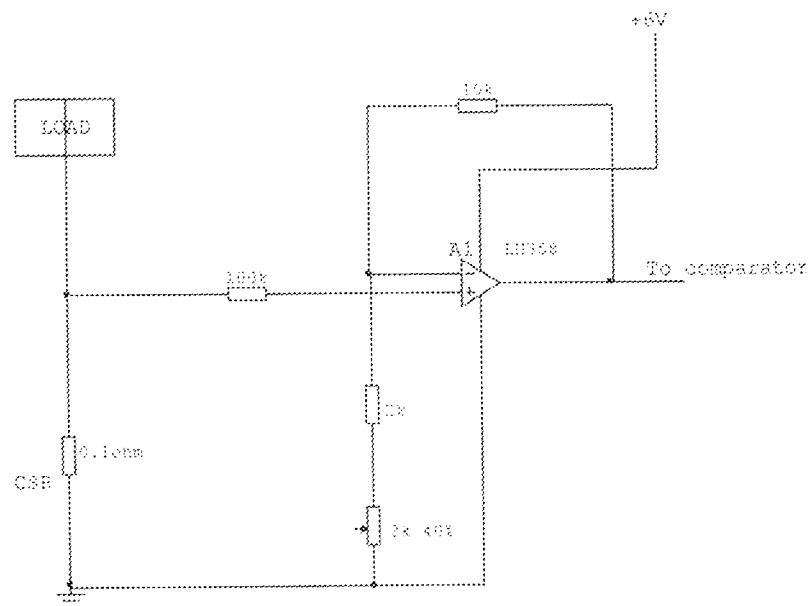
Fig. 3.2 Current — Voltage Converter and Amplifier.
