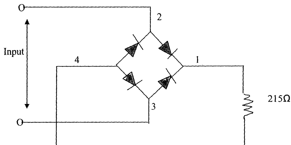
Fig. 3.3 Circuit of Bridge Rectifier
