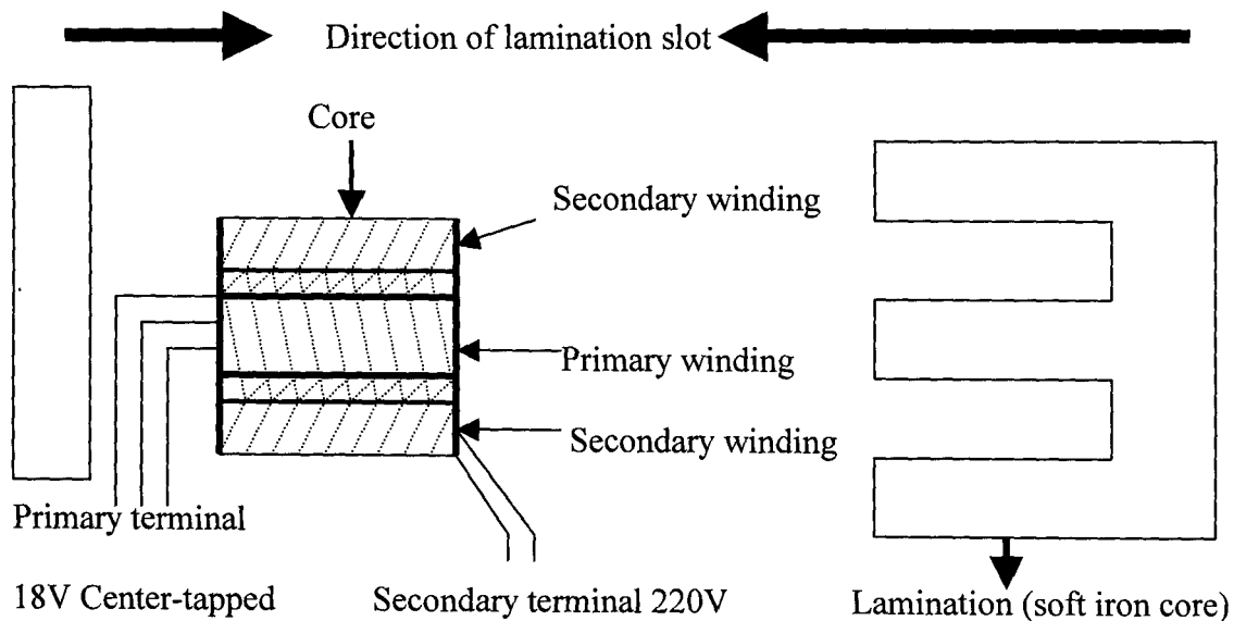
Fig 2.61 Internal Architecture of the step-up transformer (18V to 110V)
