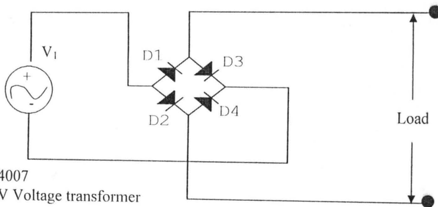
Fig. 3.1 Full-wave Bridge Rectifier
