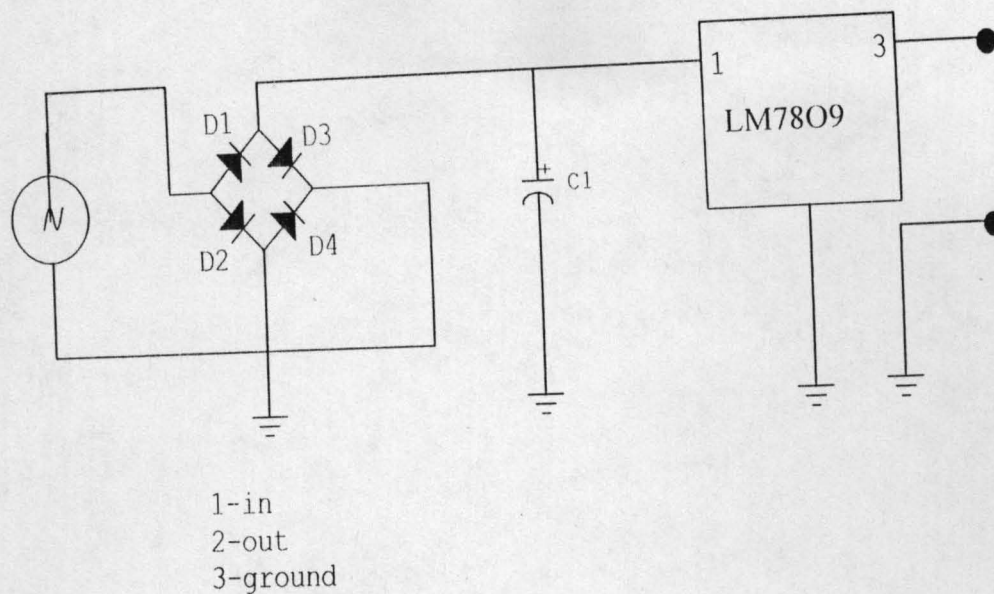
Fig: 3.3 Regulated D.C Power Supply
