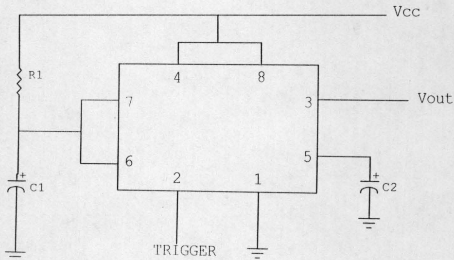
Fig: 3.7 Monostable timer circuit
