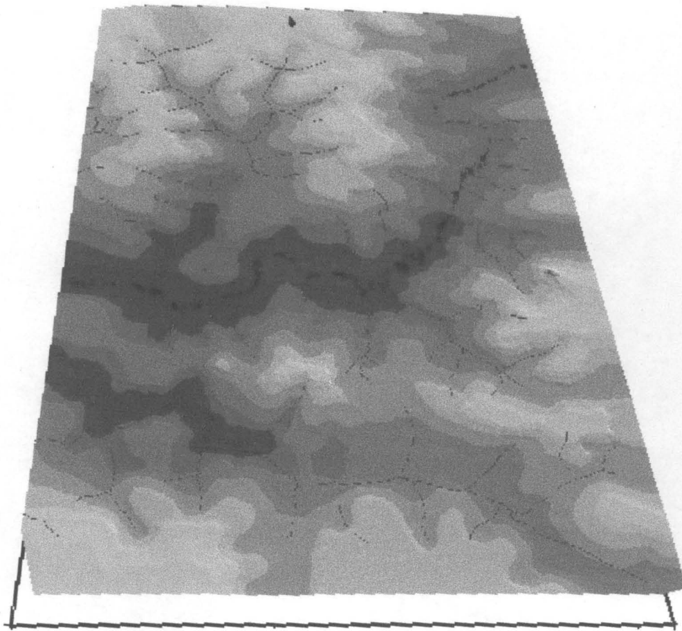
Fig. 4.8: Digital Elevation Model (DEM) of Kaduna Metropolis (Adapted from Topographic Map 1972) and GPS Heights (2005).
