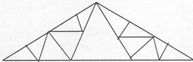
(b) French Truss
