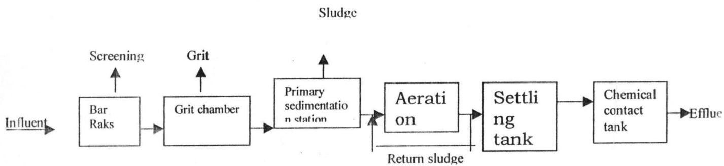
Fig 3: Simplified flow diagrams for activated sludge process
