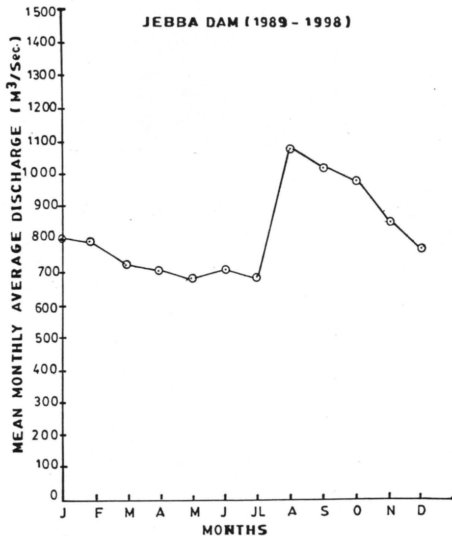
Fig.13 15 a : MEAN MONTHLY AVERAGE DISCHARGE (M 3 /Sec.) FOR TEN YEARS (1989-1998) AT JEBBA DAM ( POST DAM ) -
