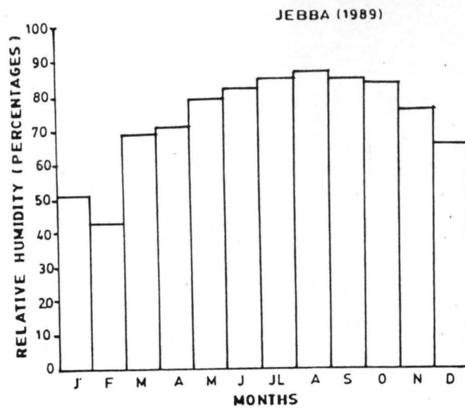
Fig. 9(a) HISTOGRAM OF RELATIVE HUMIDITY AT JEBBA DAM
