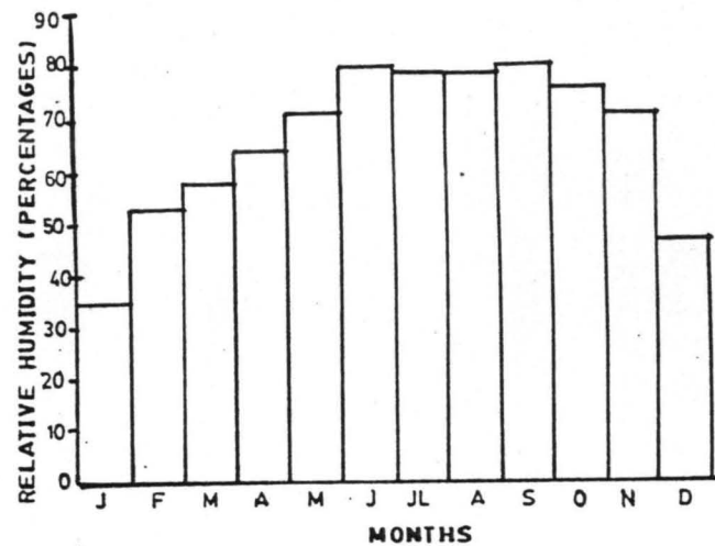
Fig. 9c HISTOGRAM OF RELATIVE HUMIDITY AT JEBBA DAM (1993)
