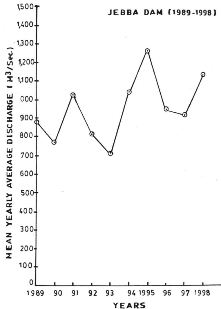
Fig.13 b : MEAN YEARLY AVERAGE DISCHARGE (M 3 /Sec.) FOR TEN YEARS (1989-1998) POST DAM -
