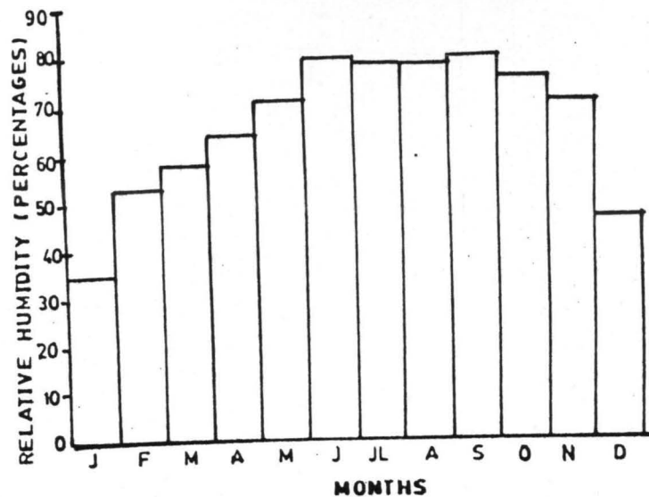
Fig-9(e) HISTOGRAM OF RELATIVE HUMIDITY AT JEBBA DAM (1993)
