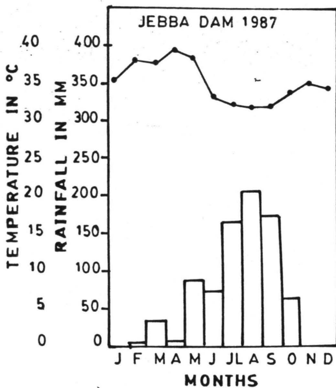
Fig-10a-j MEAN MONTHLY RAINFALL IN MM AND MEAN MONTHLY MAXIMUM TEMPERATURE (°C)
