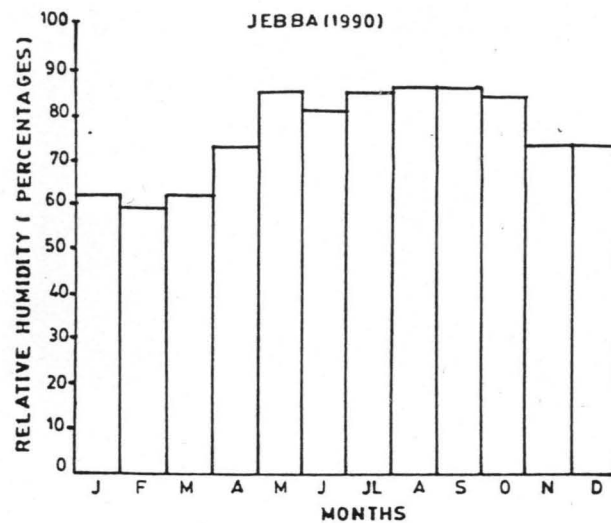
Fig. 9 b HISTOGRAM OF RELATIVE HUMIDITY AT JEBBA DAM
