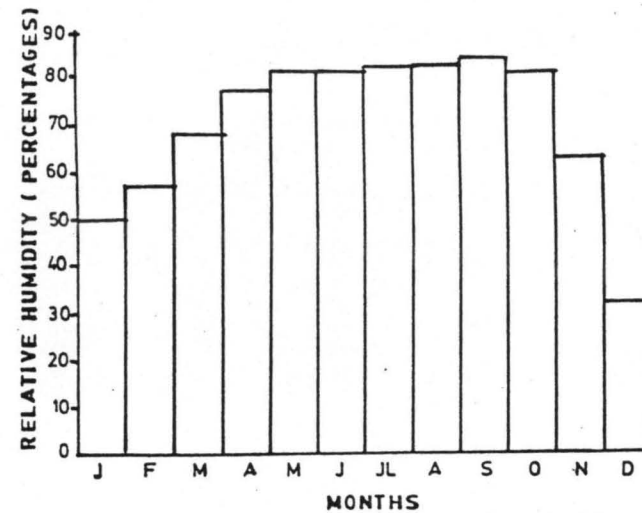
Fig. 9f HISTOGRAM OF RELATIVE HUMIDITY AT JEBBA DAM (1994)
