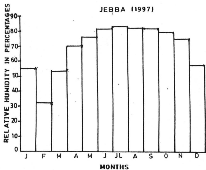
Fig.9i HISTOGRAM OF RELATIVE HUMIDITY AT JEBBA DAM
