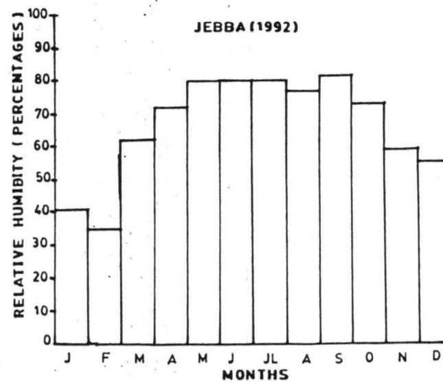
Fig. 9(d) HISTOGRAM OF RELATIVE HUMIDITY AT JEBBA DAM
