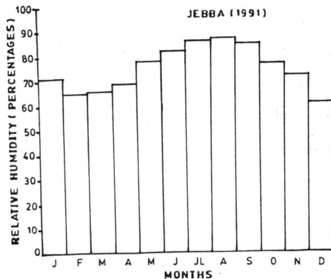
Fig. 9(c) HISTOGRAM OF RELATIVE HUMIDITY AT JEBBA DAM
