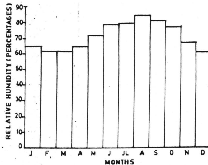
Fig-9(h) HISTOGRAM OF RELATIVE HUMIDITY AT JEBBA DAM (1996)
