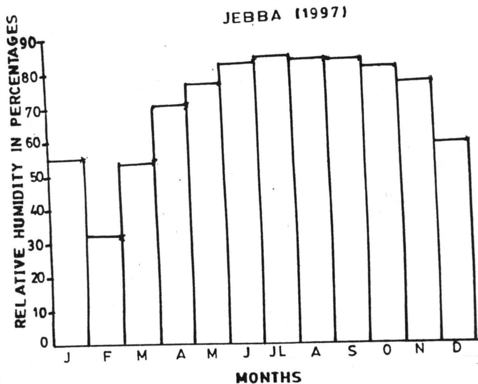
Fig.9(ii) HISTOGRAM OF RELATIVE HUMIDITY AT JEBBA DAM
