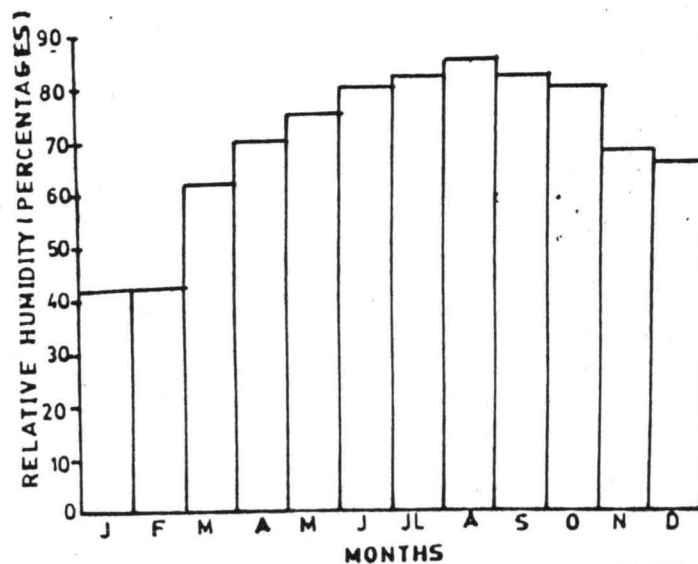
Fig-9(g) HISTOGRAM OF RELATIVE HUMIDITY AT JEBBA DAM (1995)
