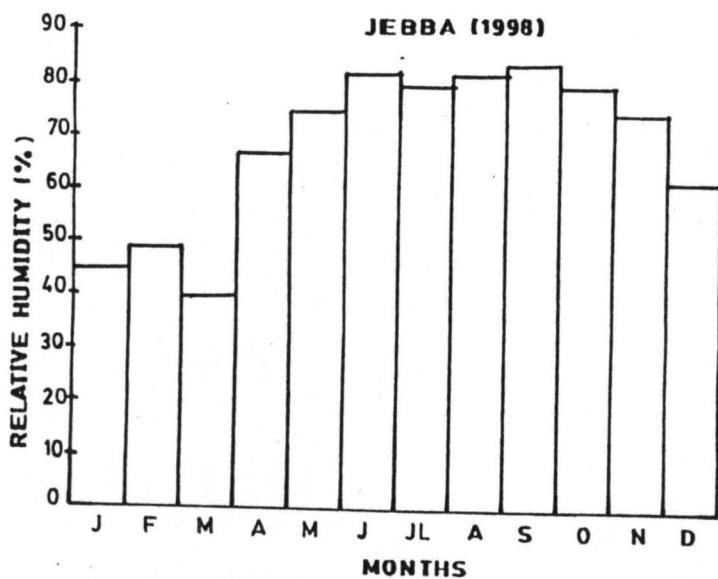
Fig.9j HISTOGRAM OF RELATIVE HUMIDITY AT JEBBA DAM
