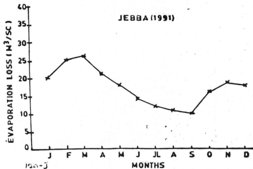
Fig-12c EVAPORATION LOSS (m³/sc) AT JEBBA DAM
