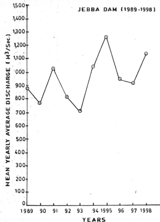
Fig. 14b MEAN YEARLY AVERAGE DISCHARGE (M³/Sec.) FOR TEN YEARS (1989-1998) POST DAM -
