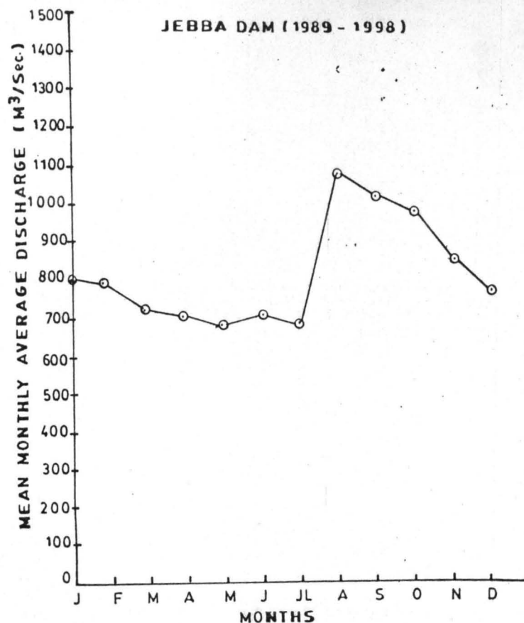
Fig. 14a MEAN MONTHLY AVERAGE DISCHARGE (M³/Sec.) FOR TEN YEARS (1989-1998) AT JEBBA DAM ( POST DAM ) -
