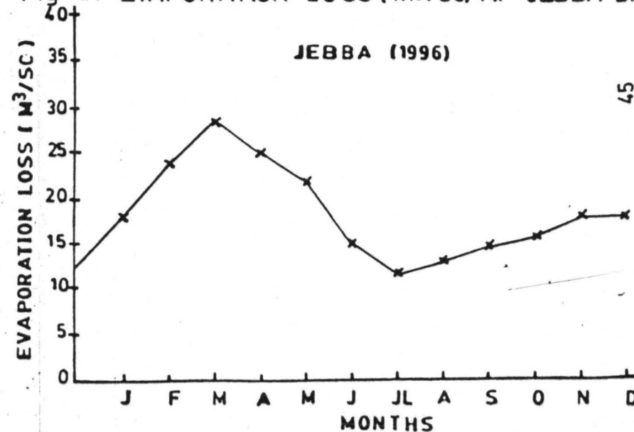
Fig.12h EVAPORATION LOSS (m³/sc) AT JEBBA DAM
