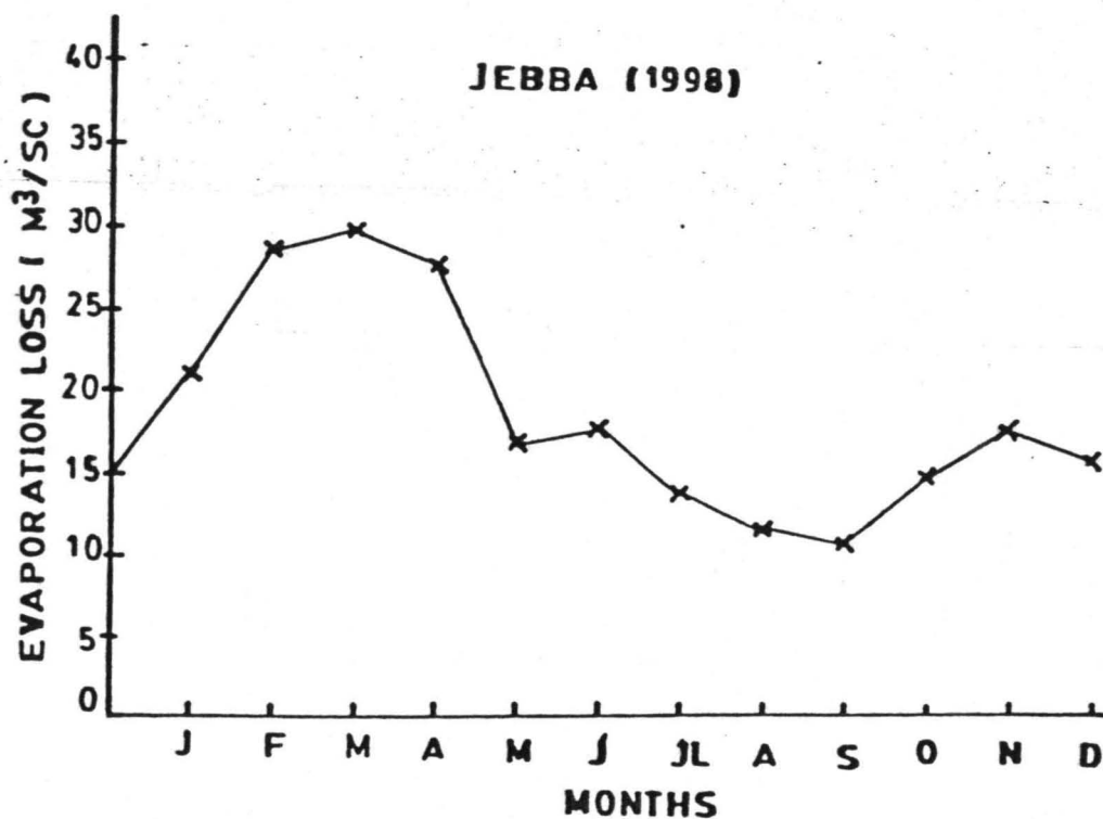
Fig.12j EVAPORATION LOSS(m³/sc.) A JEBBA DAM
