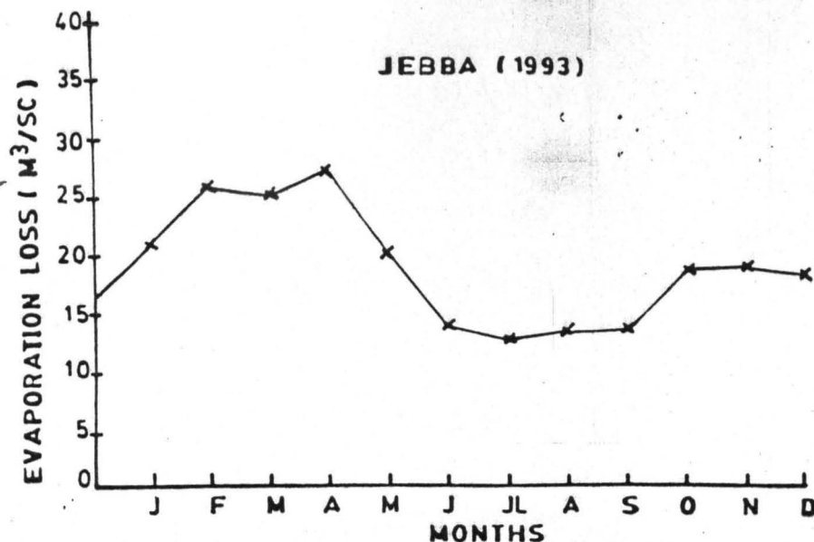
Fig.12e EVAPORATION LOSS (m³/sc) AT JEBBA DAM
