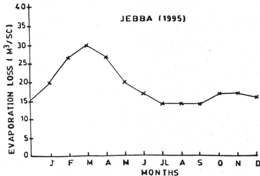
Fig.12g EVAPORATION LOSS (m³/sc) AT JEBBA DAM
