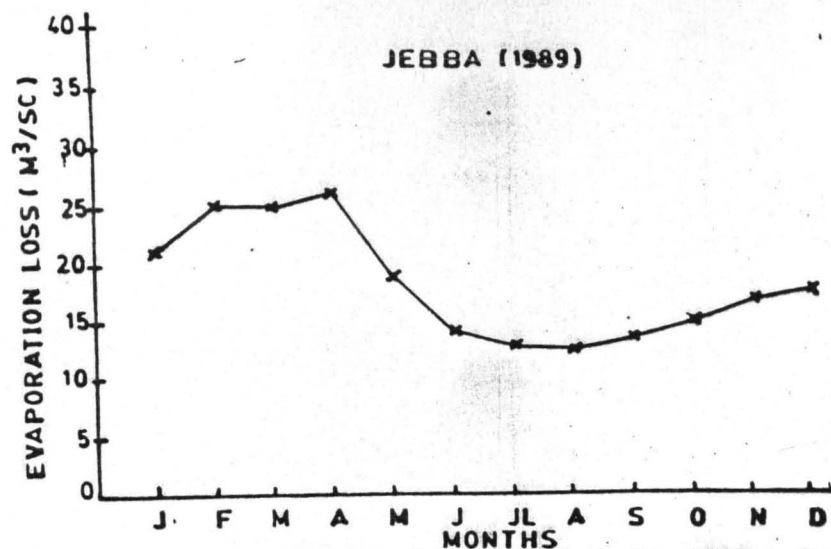
Fig-12a EVAPORATION LOSS (m³/sc) AT JEBBA DAM
