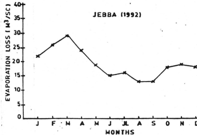
Fig-12d EVAPORATION LOSS (m³/sc) AT JEBBA DAM
