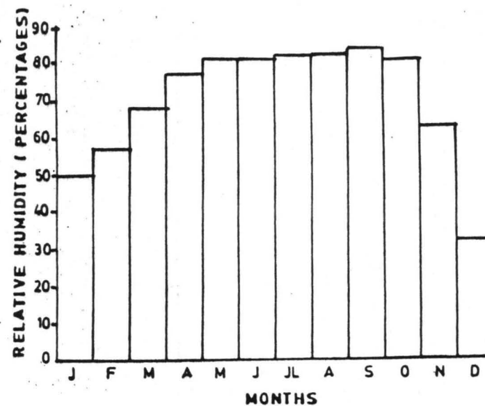
Fig-9(h) HISTOGRAM OF RELATIVE HUMIDITY AT JEBBA DAM (1994)
