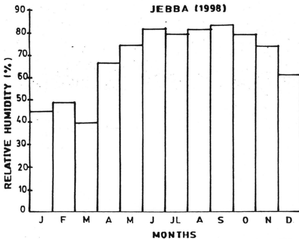
Fig.9(ij) HISTOGRAM OF RELATIVE HUMIDITY AT JEBBA DAM
