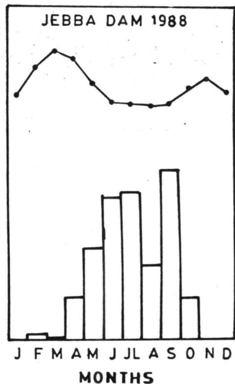
Fig-10a-j MEAN MONTHLY RAINFALL IN MM AND MEAN MONTHLY MAXIMUM TEMPERATURE (°C)
