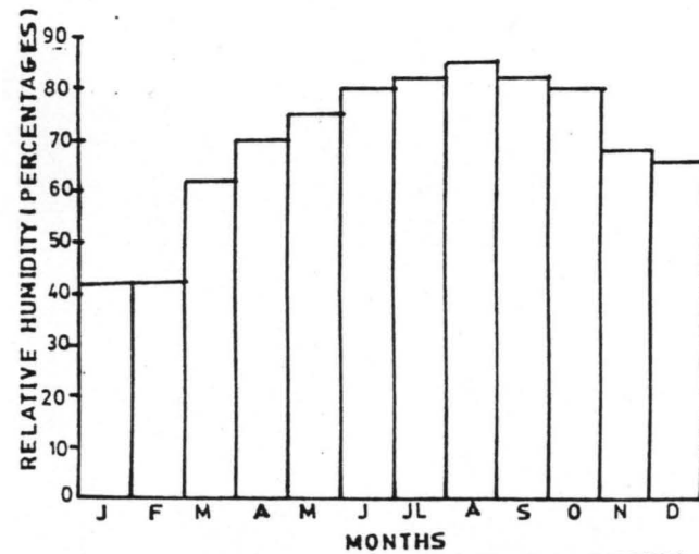
Fig. 9g HISTOGRAM OF RELATIVE HUMIDITY AT JEBBA DAM (1995)
