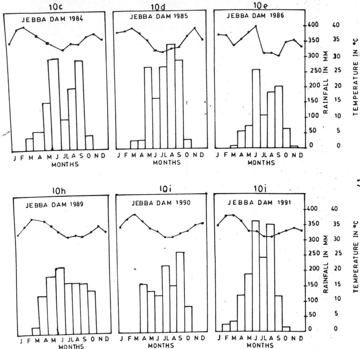
Fig-10a-j MEAN MONTHLY RAINFALL IN MM AND MEAN MONTHLY MAXIMUM TEMPERATURE (°C).
