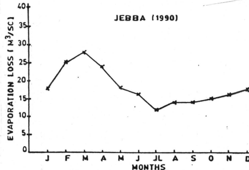
Fig-12b EVAPORATION LOSS (m³/sc) AT JEBBA DAM
