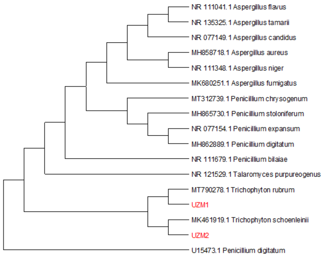
Figure 4.1: Phylogentic tree showing the relations among the fungal isolates
