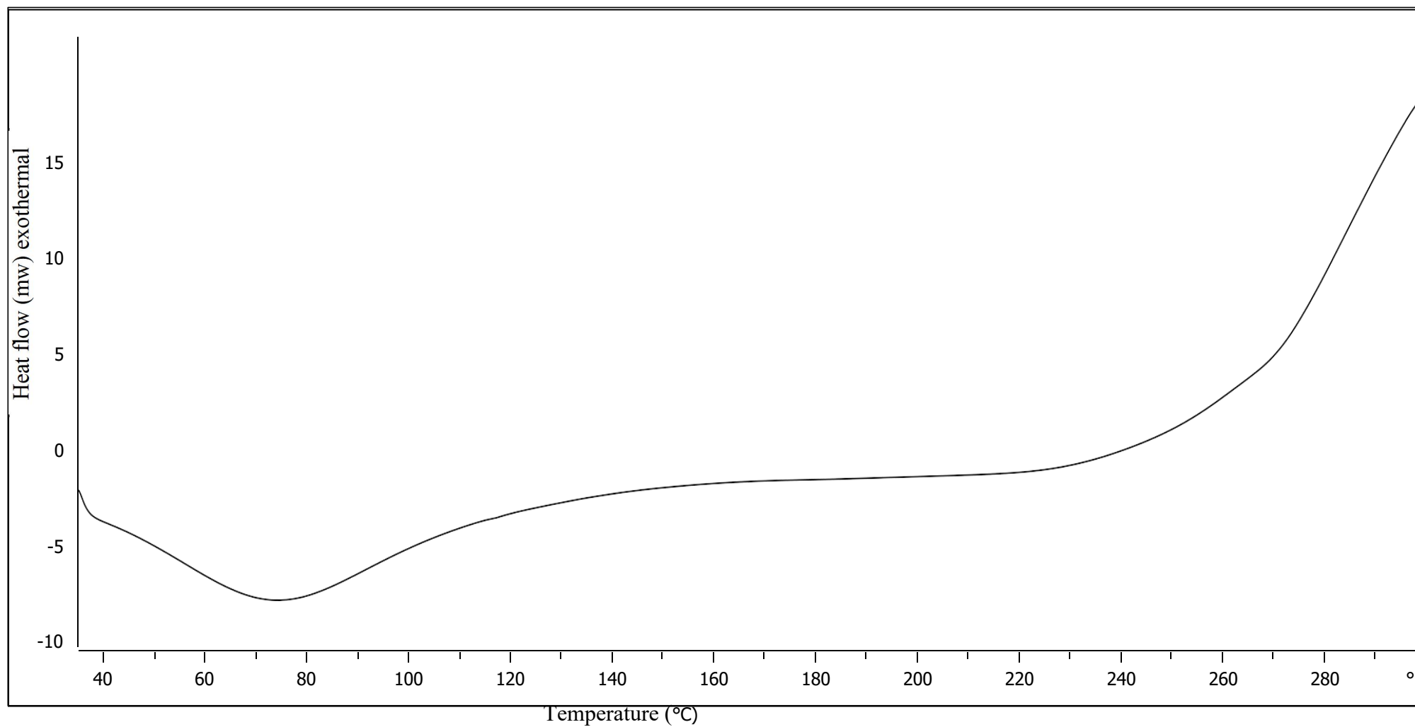
Figure 4.3a: Differential scanning calorimetry of xanthan gum produced by Stenotrophomonas maltophilia IAE12
