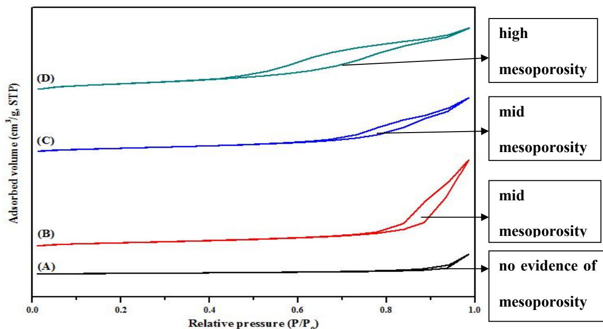
Figure 4.6: BET spectra of (a) pure \text{ZrO}_2 (b) \text{ZrO}_2\text{-S} (c) \text{ZrO}_2\text{-C} (d) \text{ZrO}_2\text{-S-C}
