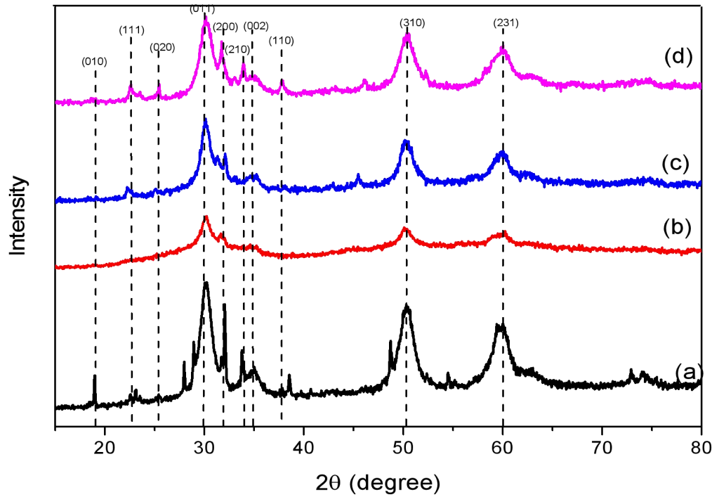
Figure 4.2: XRD pattern of (a) \text{ZrO}_2 (b) \text{ZrO}_2 doped with 3% sulphur (c) \text{ZrO}_2 doped with 3% carbon (d) \text{ZrO}_2 co-doped with 3% carbon and sulphur.
