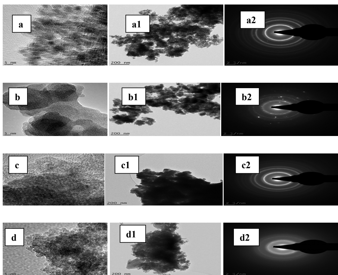
Plate III: HRTEM images at low and high magnification and selected SAED pattern of (a) pure \text{ZrO}_2 (b) 3% sulphur doped \text{ZrO}_2 (c) 3% carbon doped \text{ZrO}_2 (d) 3% carbon-sulphur doped \text{ZrO}_2
