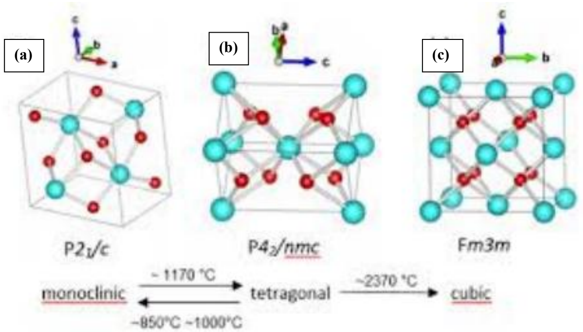
Figure: 2.2 Crystal structure of (a) monoclinic (b) tetragonal (c) cubic phase of \text{ZrO}_2 (Sigwadi et al. , 2017).
