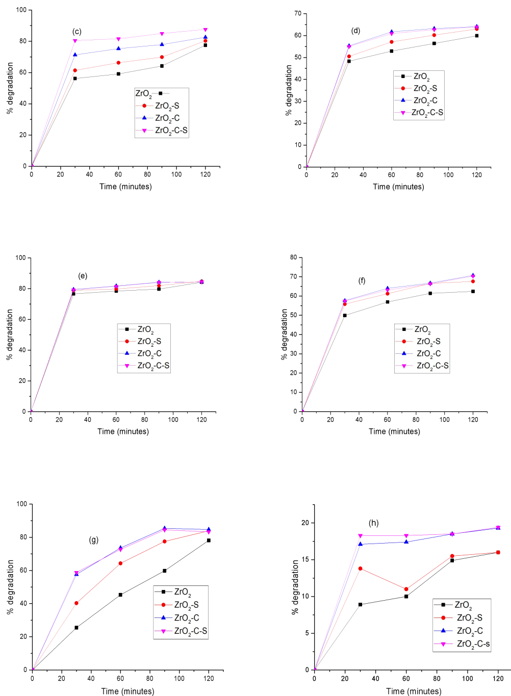
Figure 4.8: Percentage removal efficiency (a) TOC (b) COD (c) BOD (d) \text{SO}_4^{2-} (e) \text{CO}_3^{2-} (f) \text{Cl}^- (g) \text{NO}_3^- (h) pH using (i) \text{ZrO}_2 alone (ii) \text{ZrO}_2 with 3% sulphur (iii) \text{ZrO}_2 with 3% carbon (iv) \text{ZrO}_2 with 3% carbon-sulphur.
