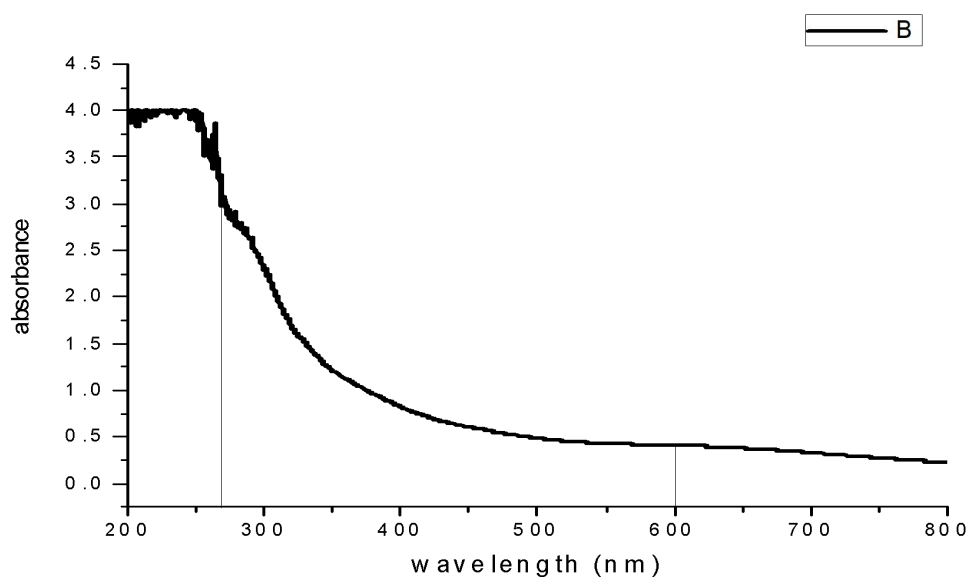
Figure 4.7: UV-visible spectra of local dye wastewater
