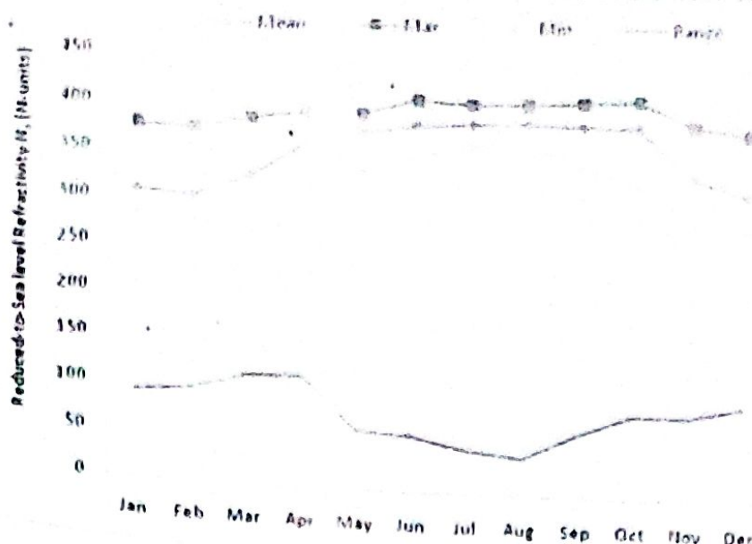
Fig. 6: Mean Monthly N_0 in Minna
