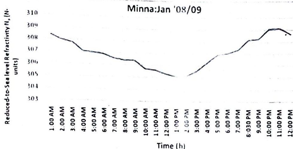
Fig. 1: Two-Year Mean Diurnal N_0 in Minna for a Typical Dry Season Month
