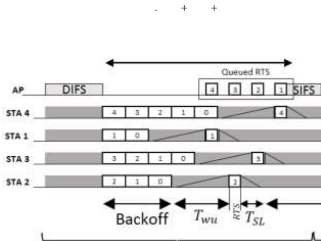
Figure 3.9 The Contention Stage of the HCA-CSMA/CA = ( + . ( . + + ) + ) + . ( . + + ) + + ) ) - \tag{3.11}
