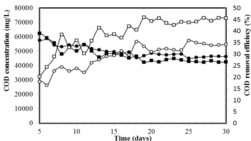
Figure 1. COD concentration and COD percentage reduction of the complete mix anaerobic reactor (■) R1 COD concentration of pre-treated OPMF + CM + POME; (□) R1 COD removal efficiency; (●) R2 COD Untreated OPMF + CM + POME (○) COD removal efficiency.
